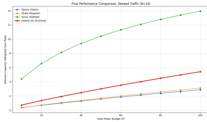
Figure 8: Architecture Comparison under Skewed Traffic using Shannon Capacity
