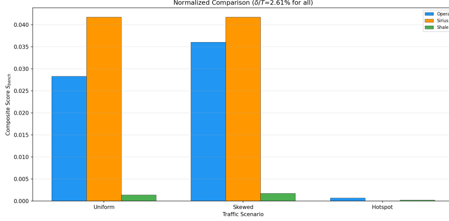
Figure 29: Composite S_{\text{bench}} under normalized hardware ( \delta/T = 2.61\% for all). Sirius leads Uniform/Skewed; all three score near zero under Hotspot. The remaining performance differences are purely routing-structural.
