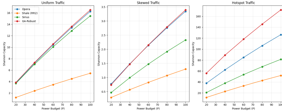
Figure 23: Topology Capacity Benchmark: Shannon Capacity vs Power Budget across different traffic models.
