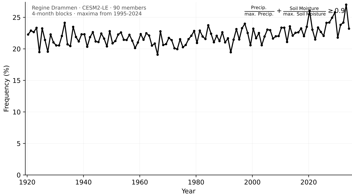
Frequency of Compound Threshold Exceedance — 2-Day Precipitation Sum + Soil-Moisture Mean, Mar-Jun, 1920-2034
