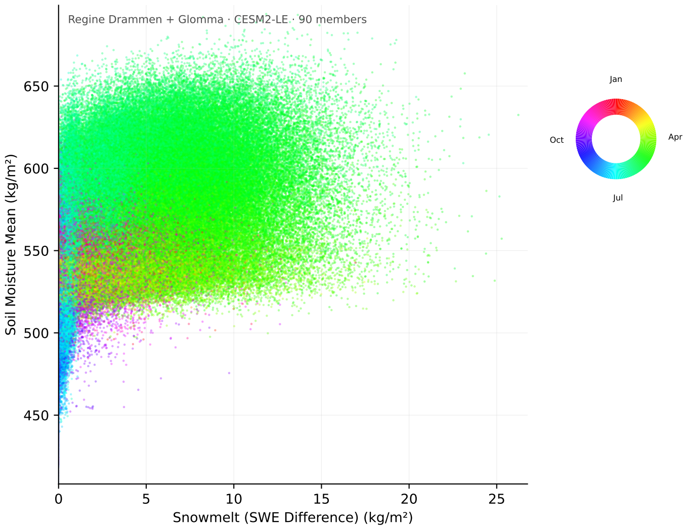
Joint Distribution of 2-Day Snowmelt (SWE Difference) and 2-Day Soil-Moisture Mean, 1995-2024
