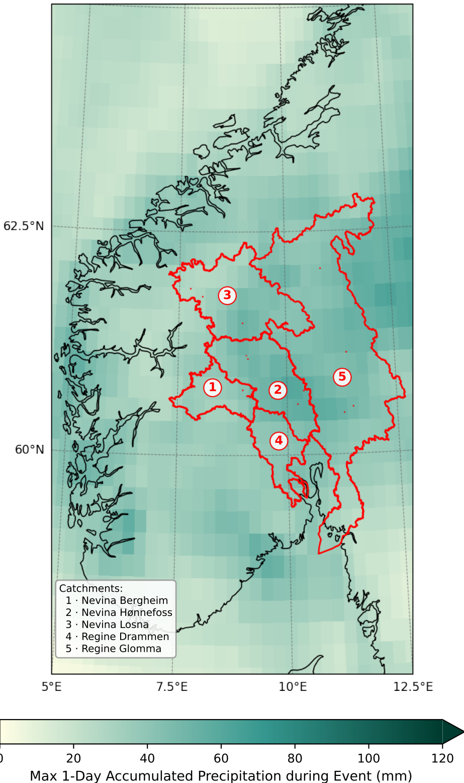
Storm Hans – Max 1-Day Precip. Envelope (7–9 Aug 2023): ERA5/0.25°x0.25°
