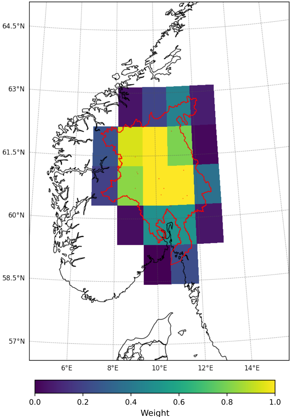
Catchment Weights: CESM2-LE/0.94x1.25 — Regime Drammen + Glomma
