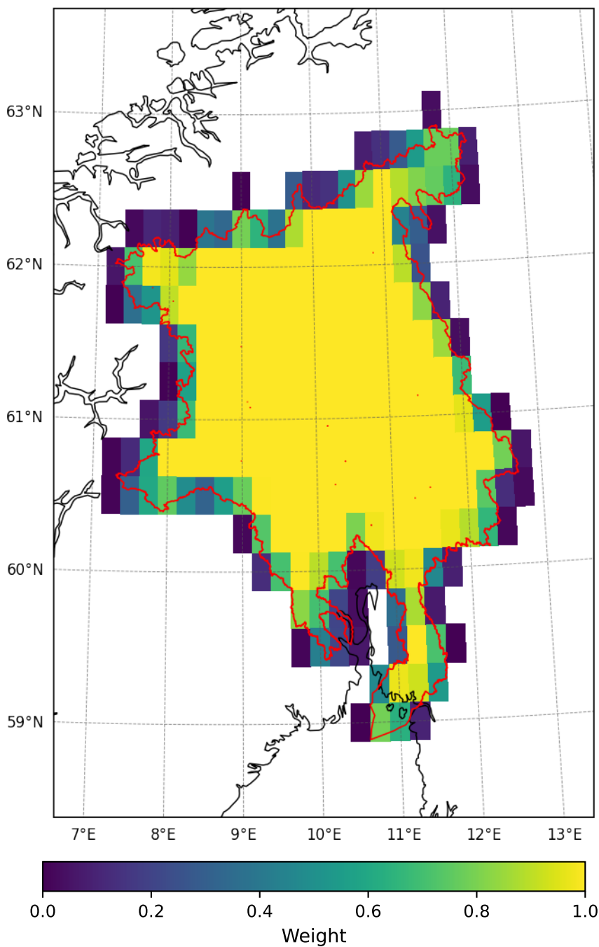
Catchment Weights: ERA5/0.25x0.25 — Regime Drammen + Glomma
