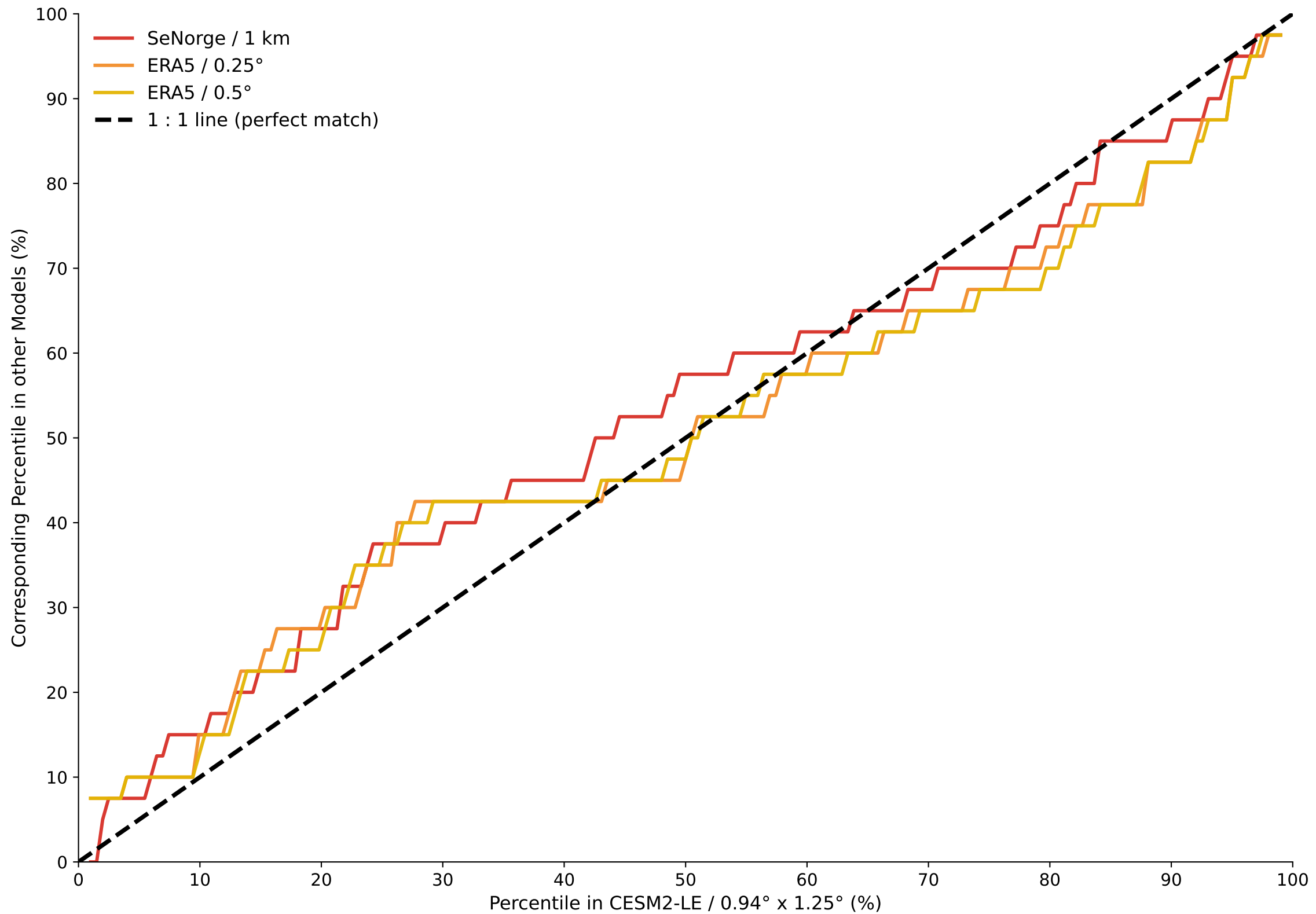
Percentile Mapping of Annual Maximal 2-day Accumulated Precipitation — Nevina Losna
