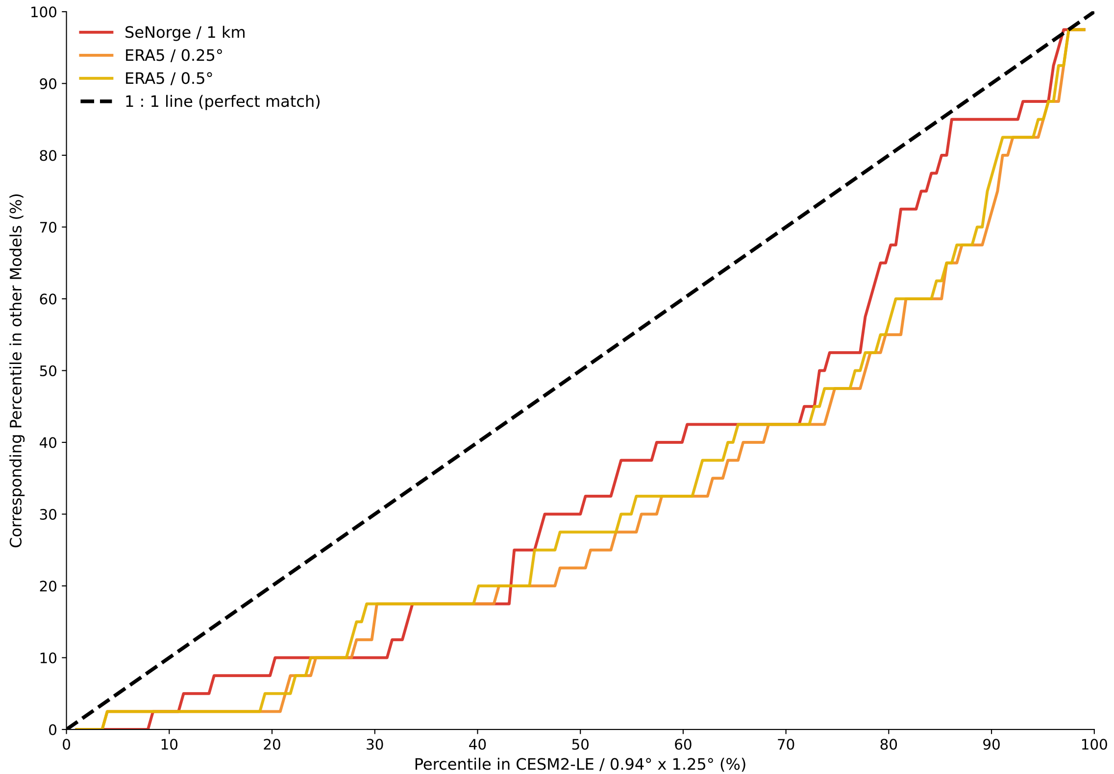
Percentile Mapping of Annual Maximal 2-day Accumulated Precipitation — Regime Drammen
