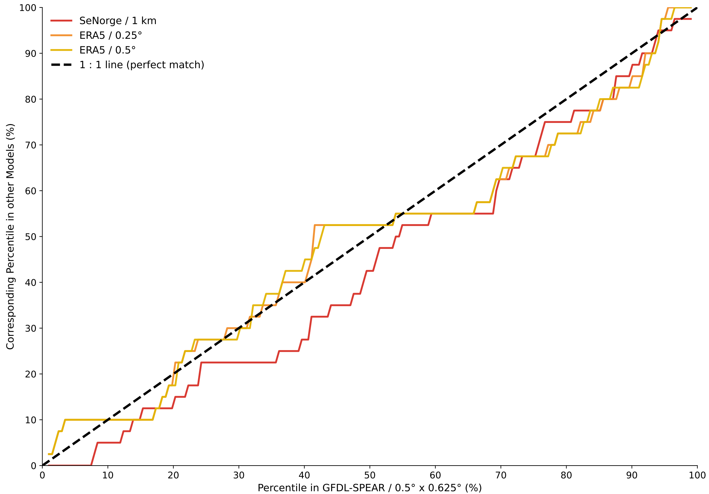
Percentile Mapping of Annual Maximal 1-day Accumulated Precipitation — Nevina Losna
