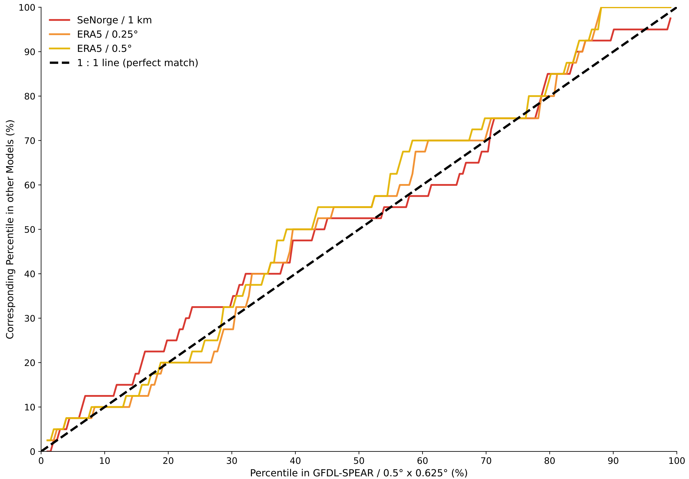
Percentile Mapping of Annual Maximal 1-day Accumulated Precipitation — Regime Drammen
