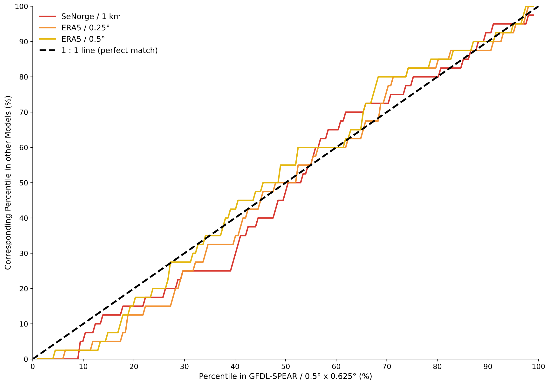
Percentile Mapping of Annual Maximal 2-day Accumulated Precipitation — Nevina Bergheim
