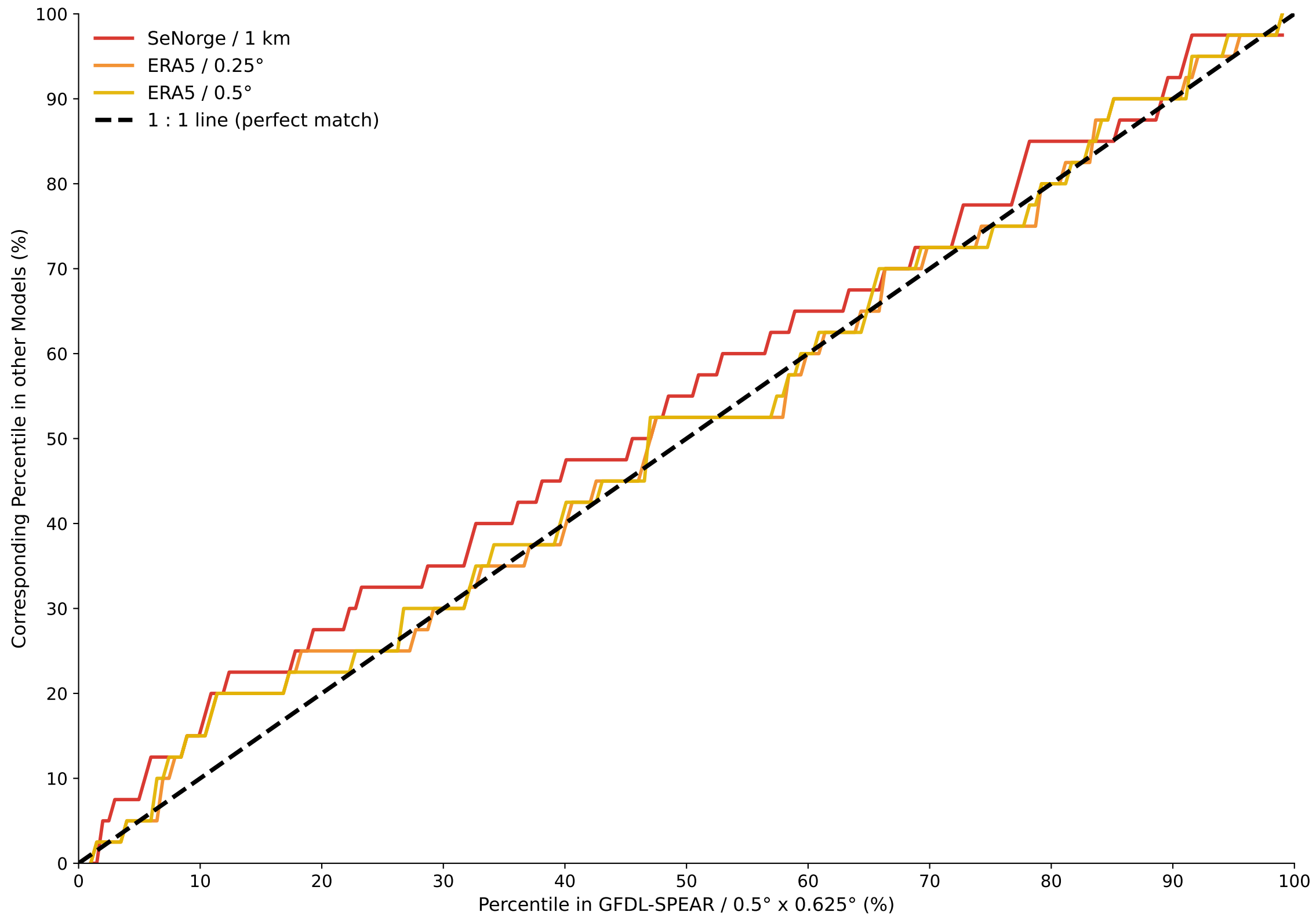
Percentile Mapping of Annual Maximal 2-day Accumulated Precipitation — Nevina Hønnefoss
