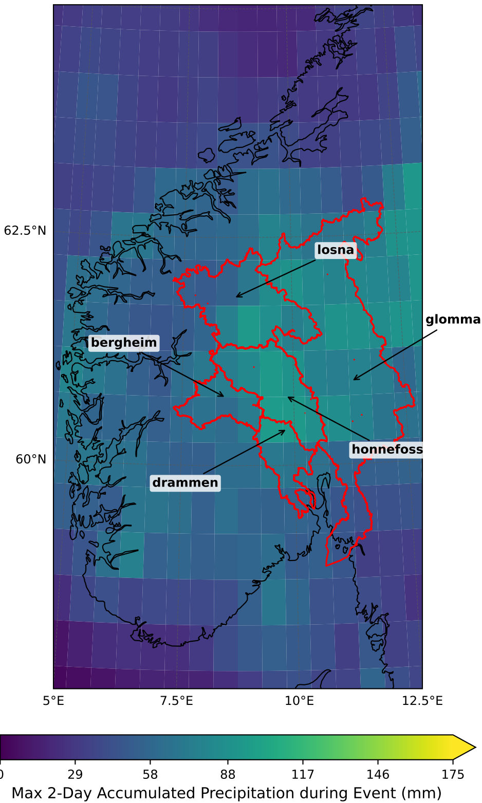
Storm Hans - Max 2-Day Precip. Envelope (7-9 Aug 2023): ERA5/0.5°x0.5°
