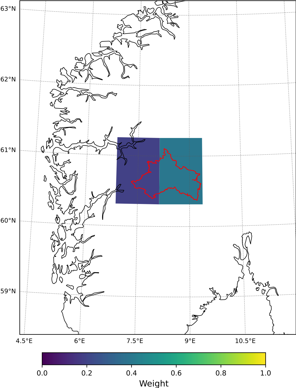
Catchment Weights: CESM2-LE/0.94x1.25 — Nevina Bergheim
