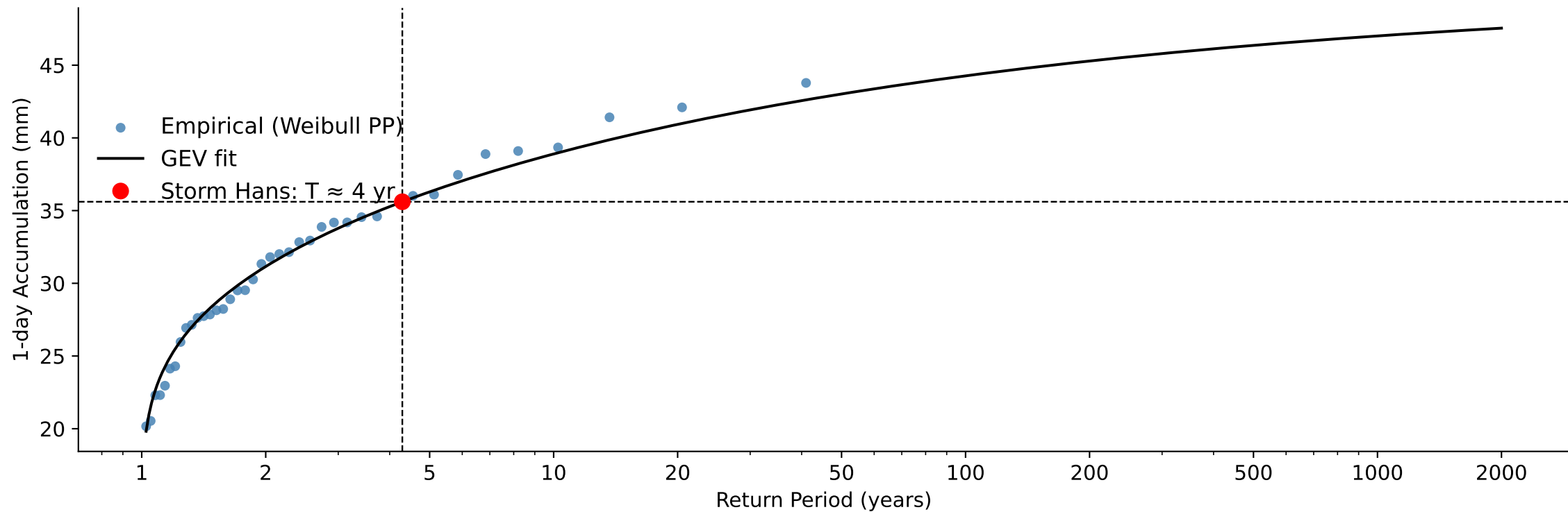
B) Weighted Catchment 1-day Accumulated Precipitation, Return Period Storm Hans: 4 year
