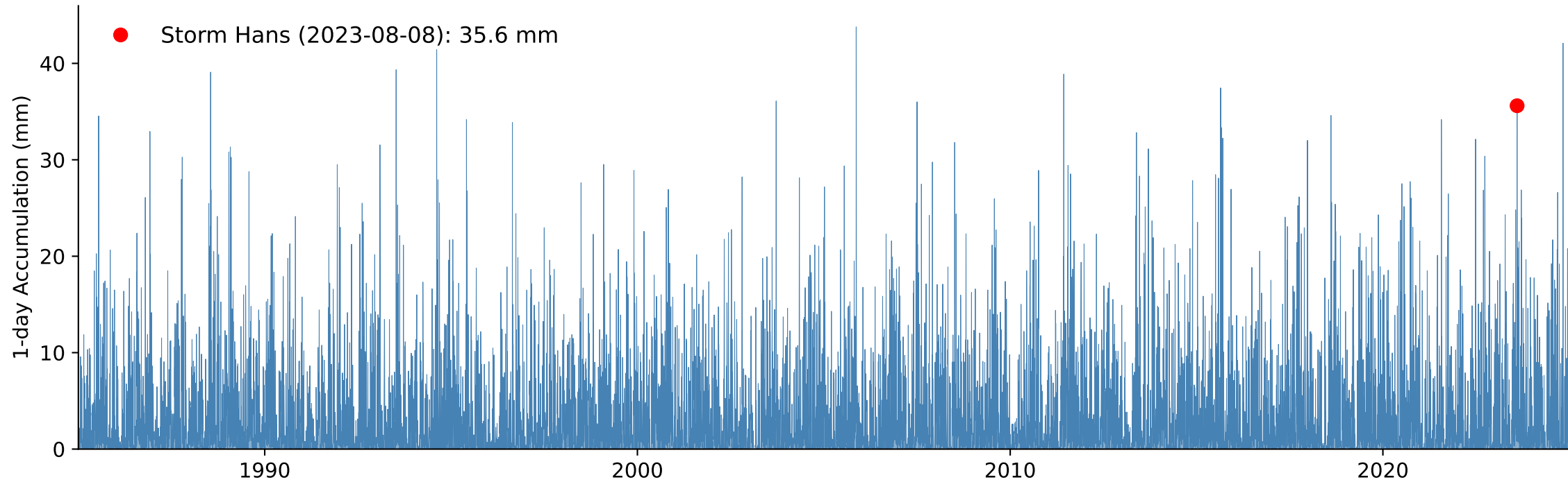
B) Weighted Catchment 1-day Accumulated Precipitation, Return Period Storm Hans: 4 year
