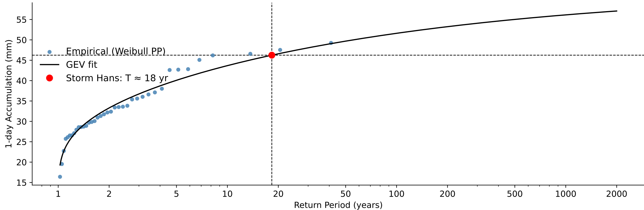
B) Weighted Catchment 1-day Accumulated Precipitation, Return Period Storm Hans: 18 year
