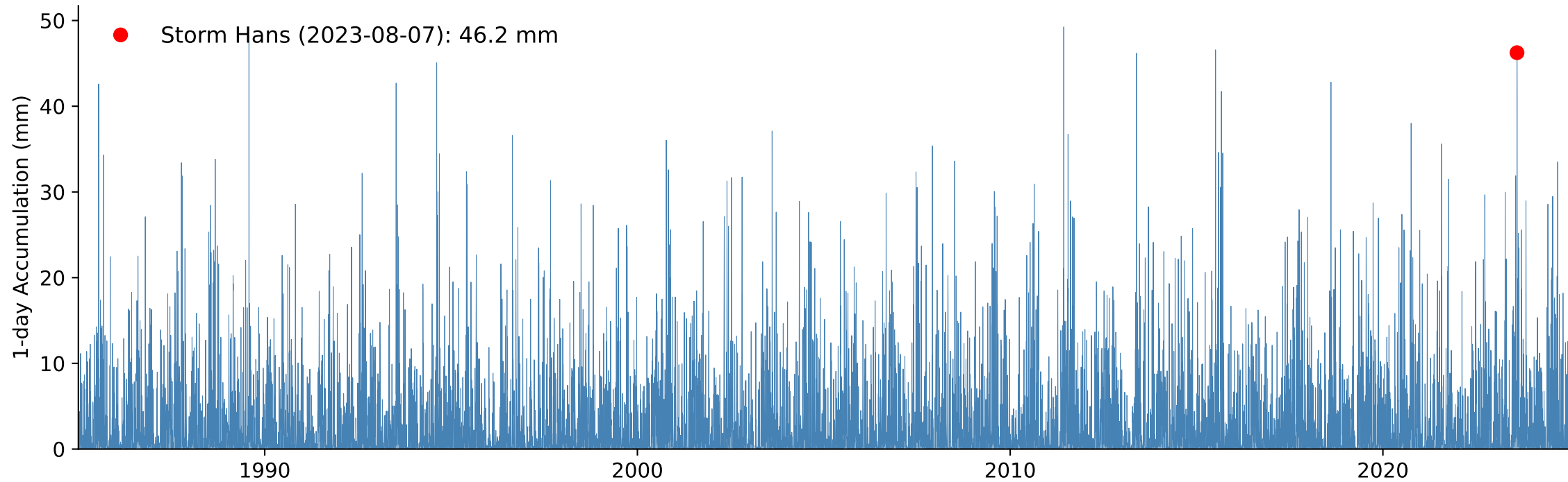
B) Weighted Catchment 1-day Accumulated Precipitation, Return Period Storm Hans: 18 year
