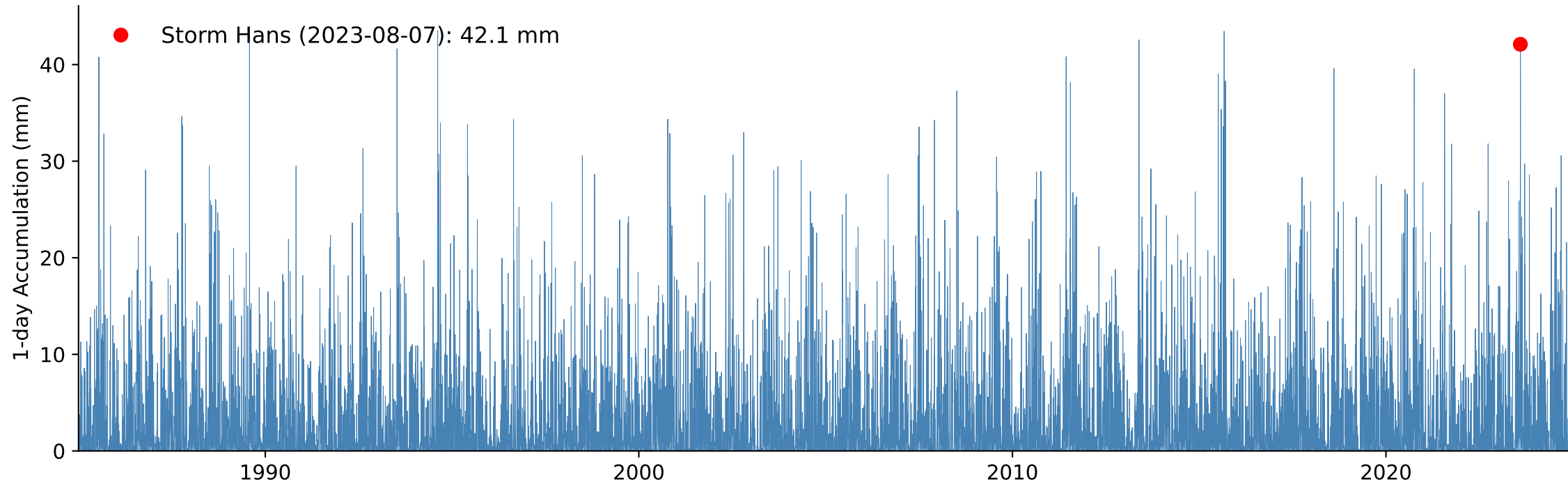
B) Weighted Catchment 1-day Accumulated Precipitation, Return Period Storm Hans: 15 year
