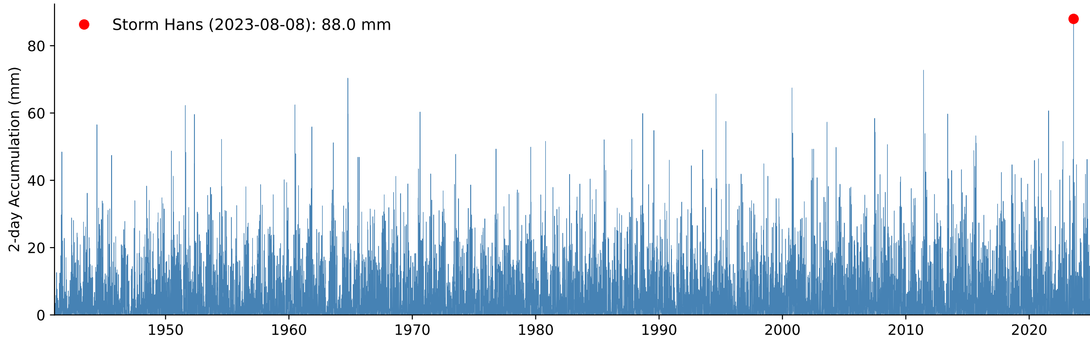
B) Weighted Catchment 2-day Accumulated Precipitation, Return Period Storm Hans: 164 year
