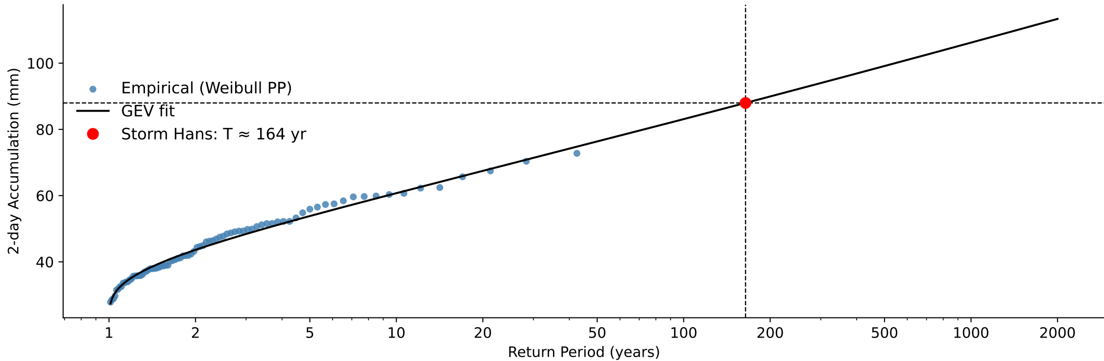
B) Weighted Catchment 2-day Accumulated Precipitation, Return Period Storm Hans: 164 year
