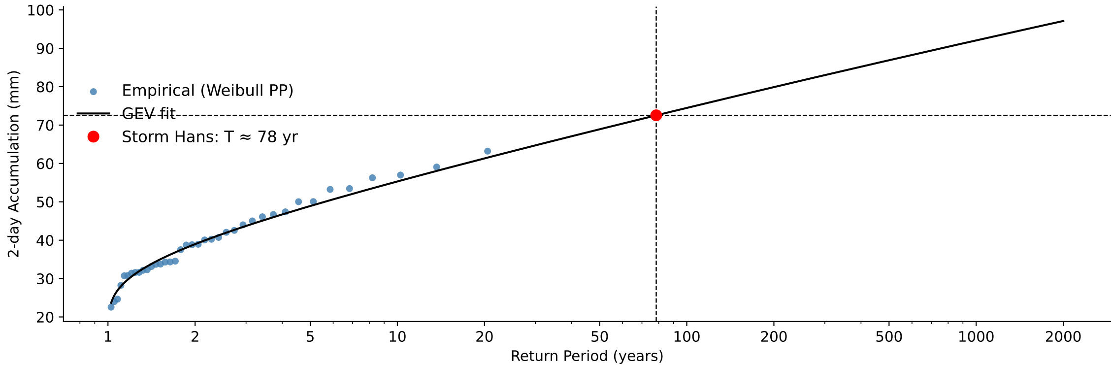
B) Weighted Catchment 2-day Accumulated Precipitation, Return Period Storm Hans: 78 year
