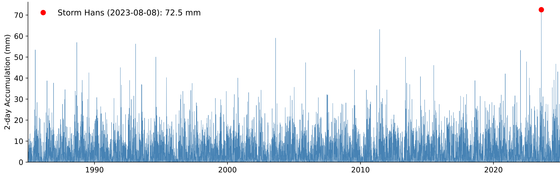
B) Weighted Catchment 2-day Accumulated Precipitation, Return Period Storm Hans: 78 year
