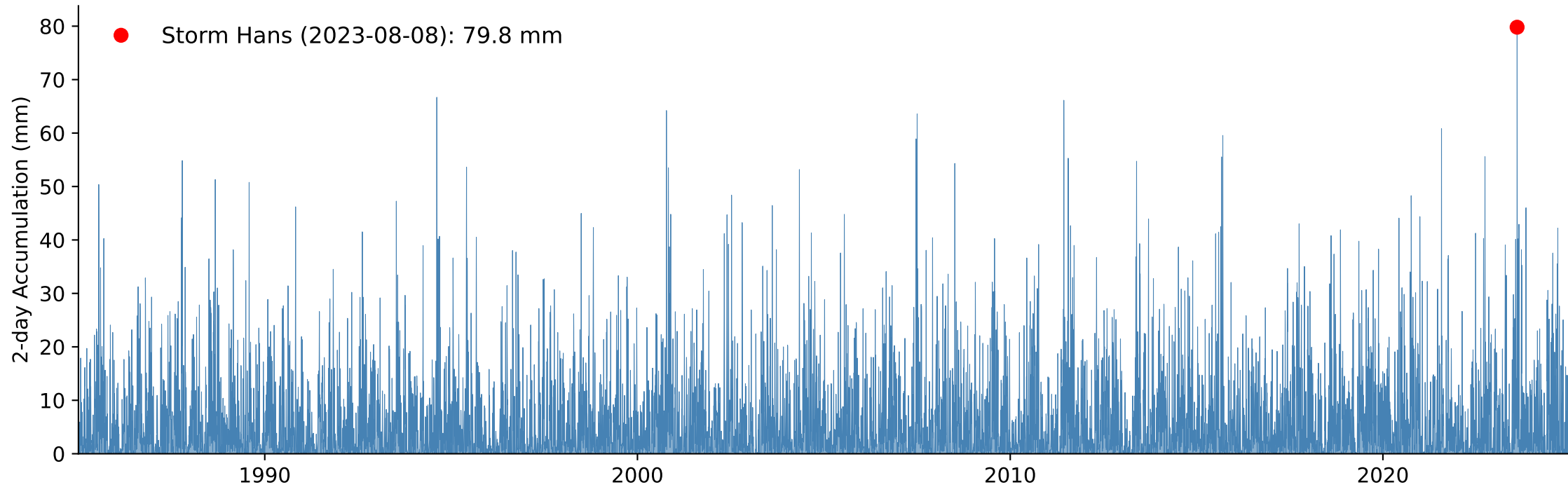
B) Weighted Catchment 2-day Accumulated Precipitation, Return Period Storm Hans: 101 year
