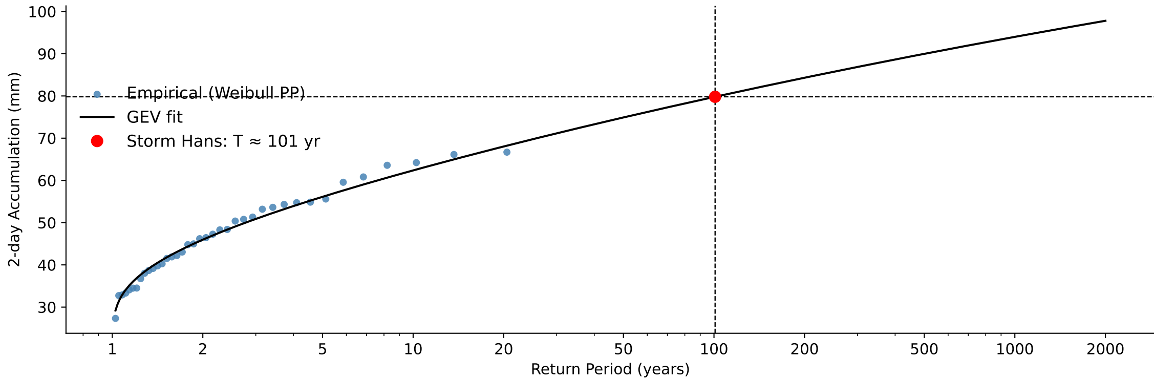
B) Weighted Catchment 2-day Accumulated Precipitation, Return Period Storm Hans: 101 year
