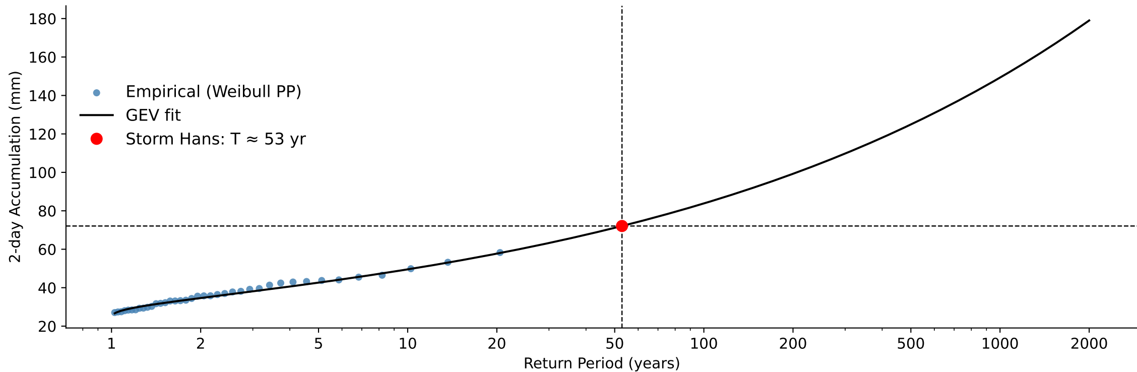
B) Weighted Catchment 2-day Accumulated Precipitation, Return Period Storm Hans: 53 year
