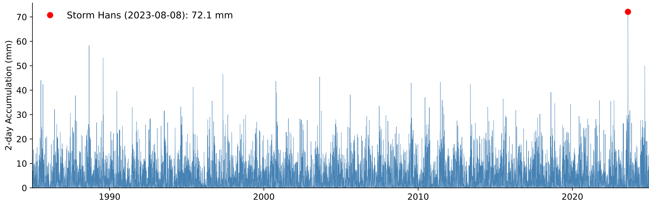
B) Weighted Catchment 2-day Accumulated Precipitation, Return Period Storm Hans: 53 year
