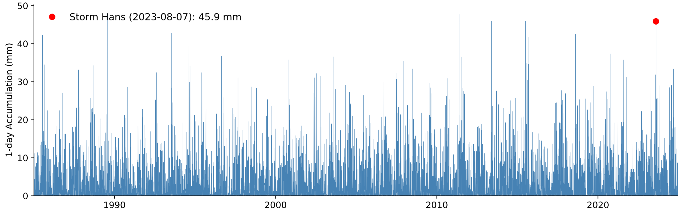
B) Weighted Catchment 1-day Accumulated Precipitation, Return Period Storm Hans: 19 year
