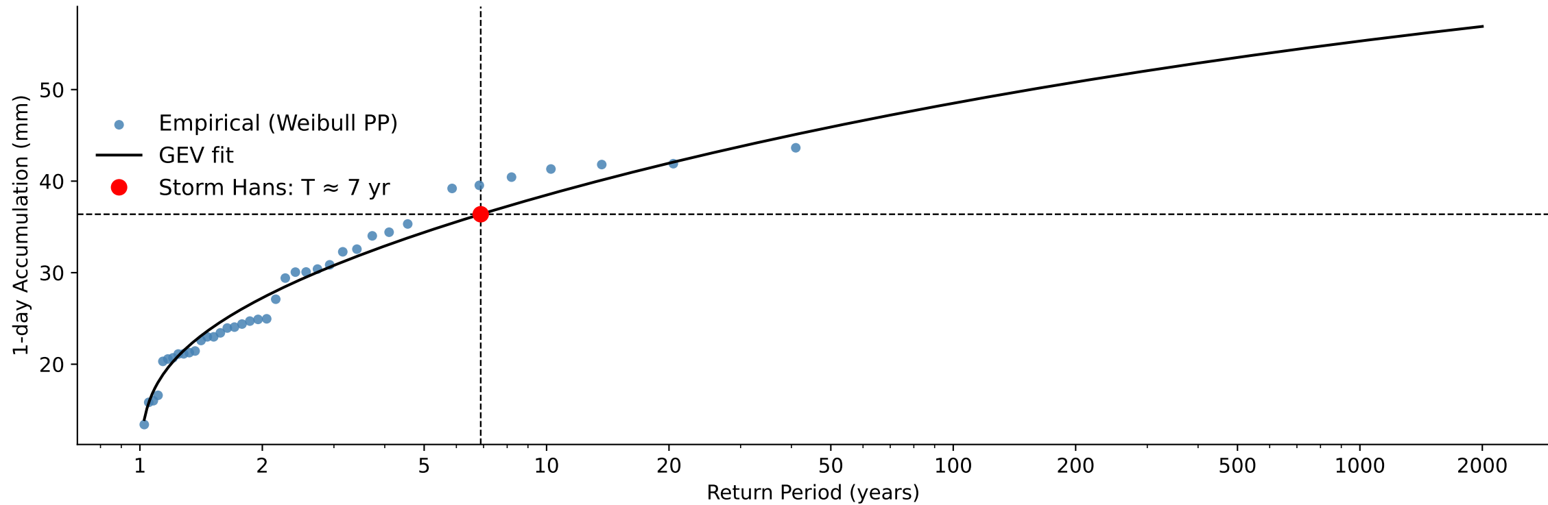
B) Weighted Catchment 1-day Accumulated Precipitation, Return Period Storm Hans: 7 year
