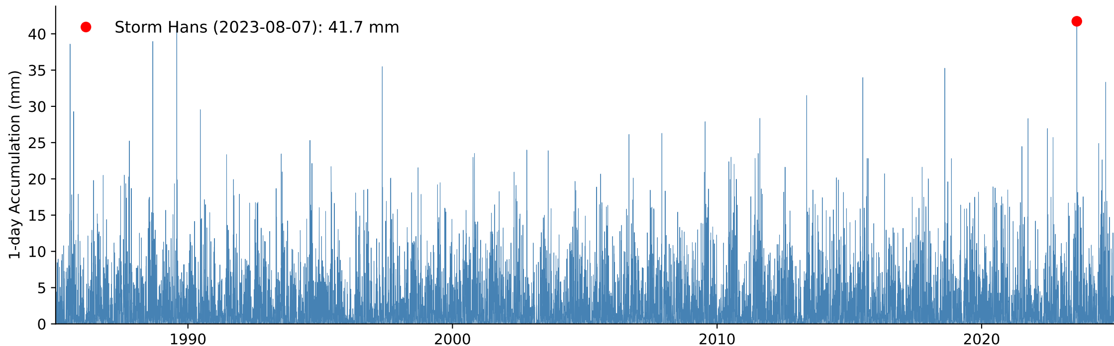
B) Weighted Catchment 1-day Accumulated Precipitation, Return Period Storm Hans: 22 year
