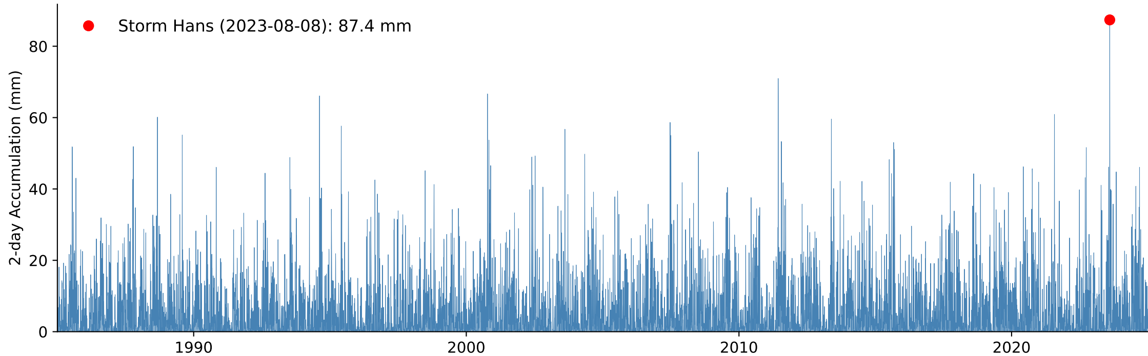
B) Weighted Catchment 2-day Accumulated Precipitation, Return Period Storm Hans: 121 year
