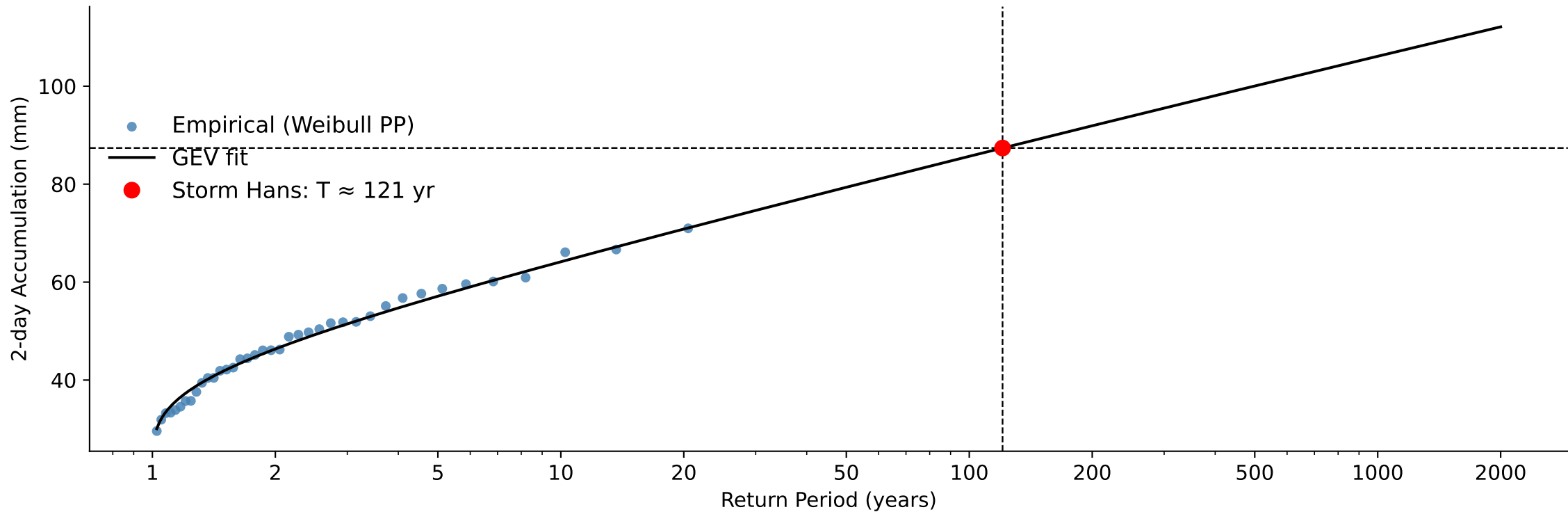
B) Weighted Catchment 2-day Accumulated Precipitation, Return Period Storm Hans: 121 year
