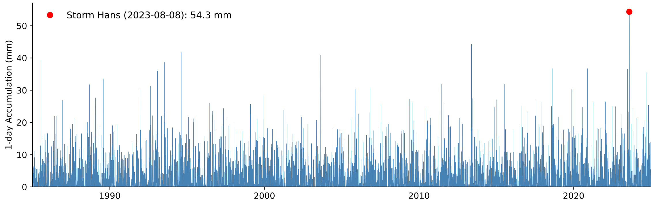
B) Weighted Catchment 1-day Accumulated Precipitation, Return Period Storm Hans: 84 year
