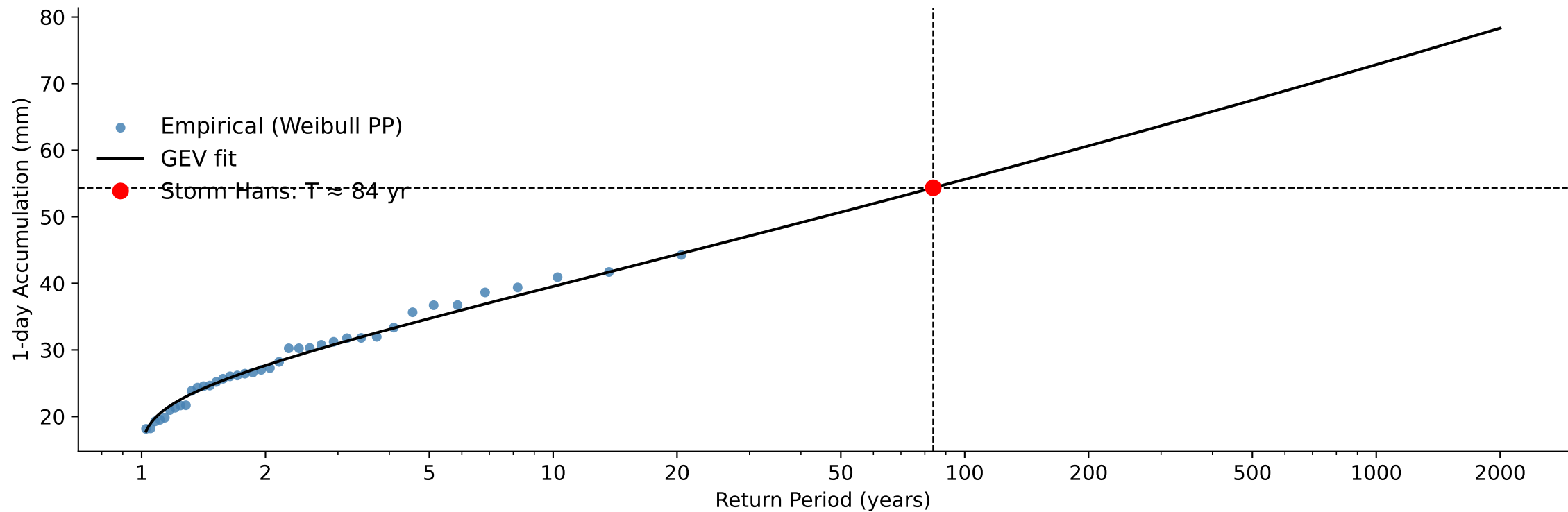
B) Weighted Catchment 1-day Accumulated Precipitation, Return Period Storm Hans: 84 year
