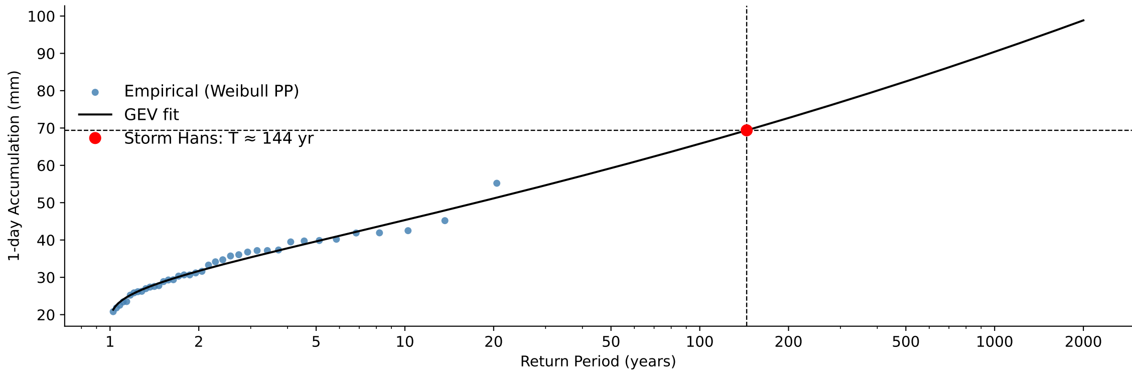
B) Weighted Catchment 1-day Accumulated Precipitation, Return Period Storm Hans: 144 year
