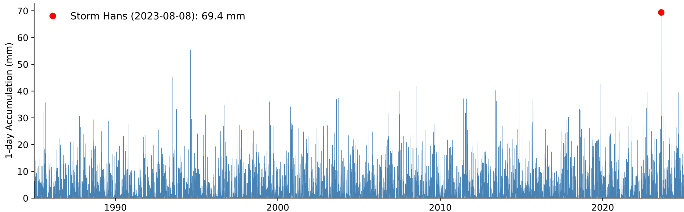
B) Weighted Catchment 1-day Accumulated Precipitation, Return Period Storm Hans: 144 year
