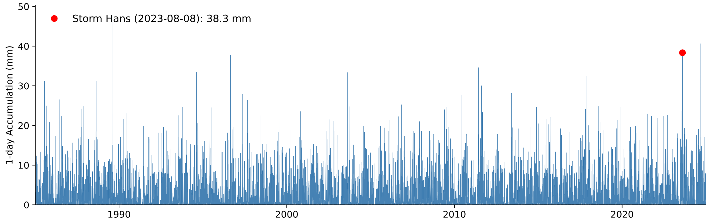
B) Weighted Catchment 1-day Accumulated Precipitation, Return Period Storm Hans: 18 year
