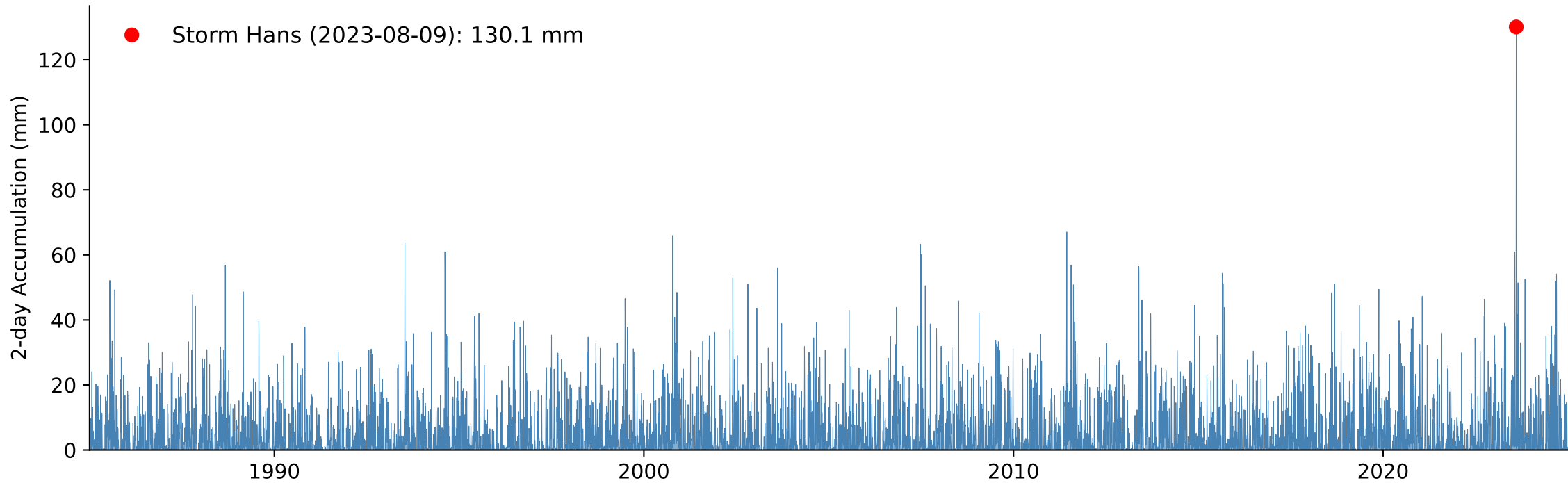
B) Weighted Catchment 2-day Accumulated Precipitation, Return Period Storm Hans: 298 year
