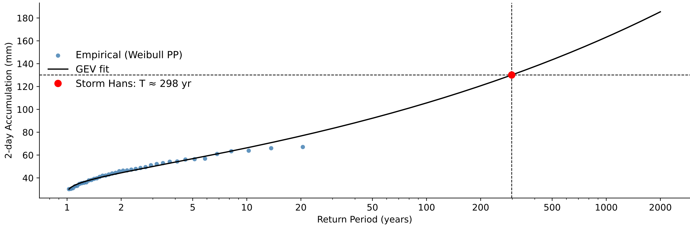
B) Weighted Catchment 2-day Accumulated Precipitation, Return Period Storm Hans: 298 year
