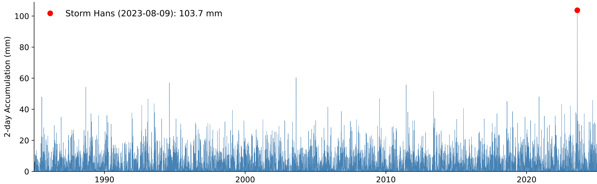
B) Weighted Catchment 2-day Accumulated Precipitation, Return Period Storm Hans: 167 year
