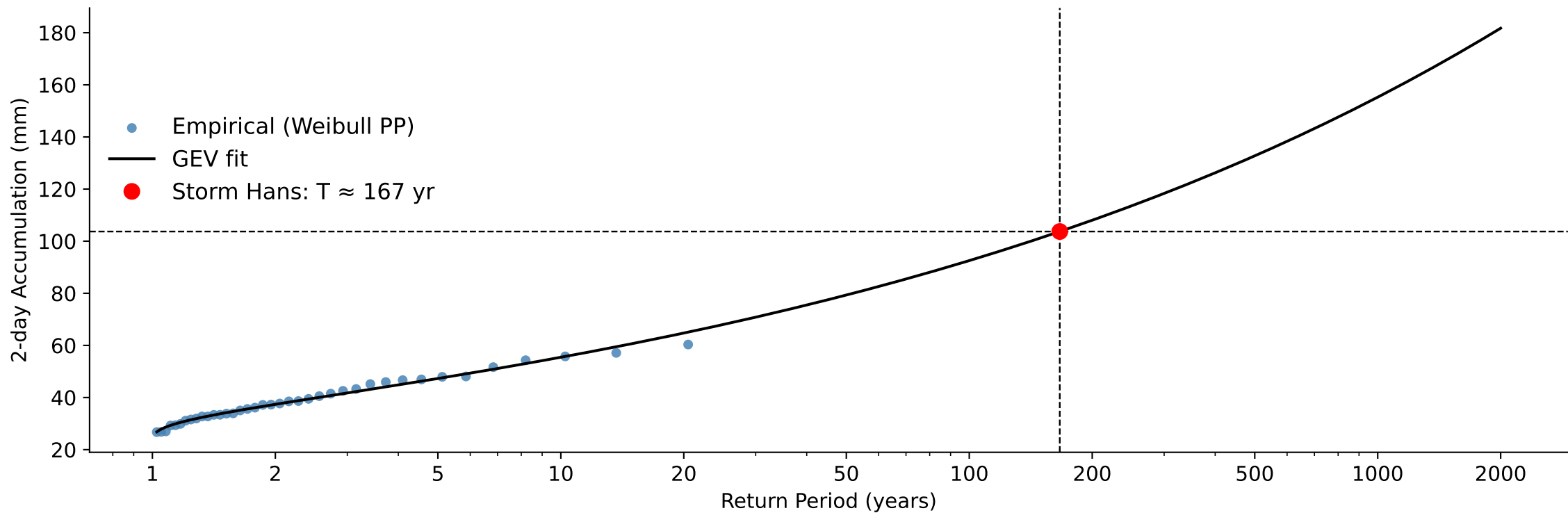
B) Weighted Catchment 2-day Accumulated Precipitation, Return Period Storm Hans: 167 year
