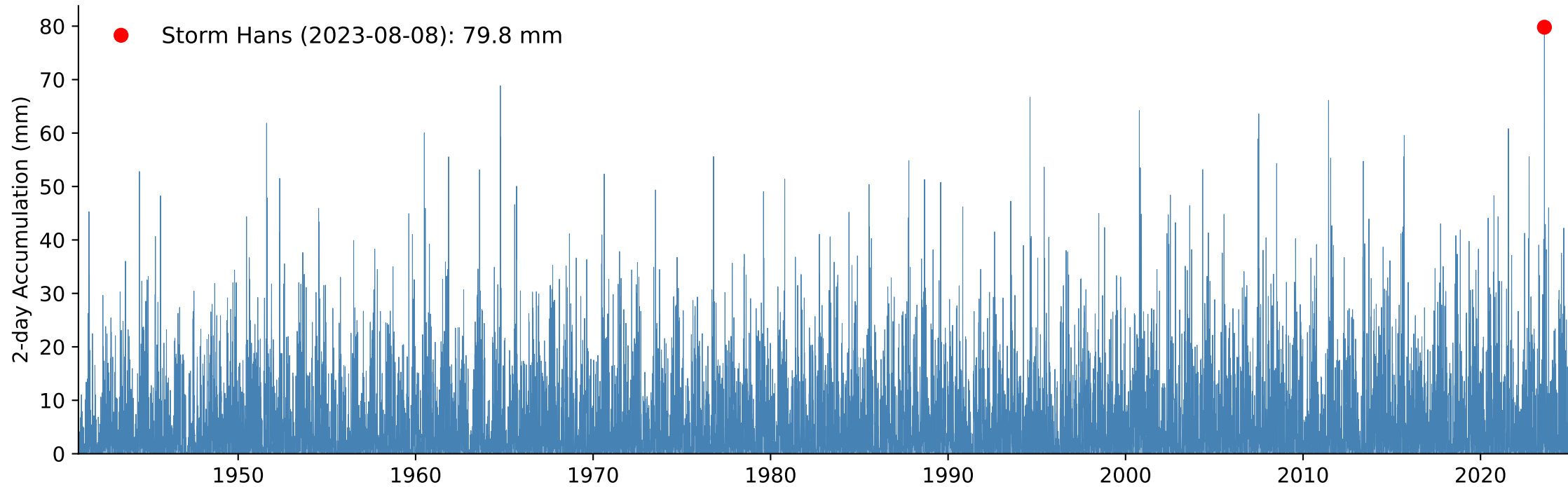
B) Weighted Catchment 2-day Accumulated Precipitation, Return Period Storm Hans: 133 year
