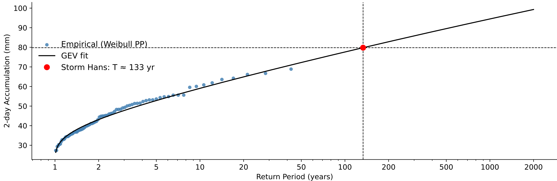
B) Weighted Catchment 2-day Accumulated Precipitation, Return Period Storm Hans: 133 year
