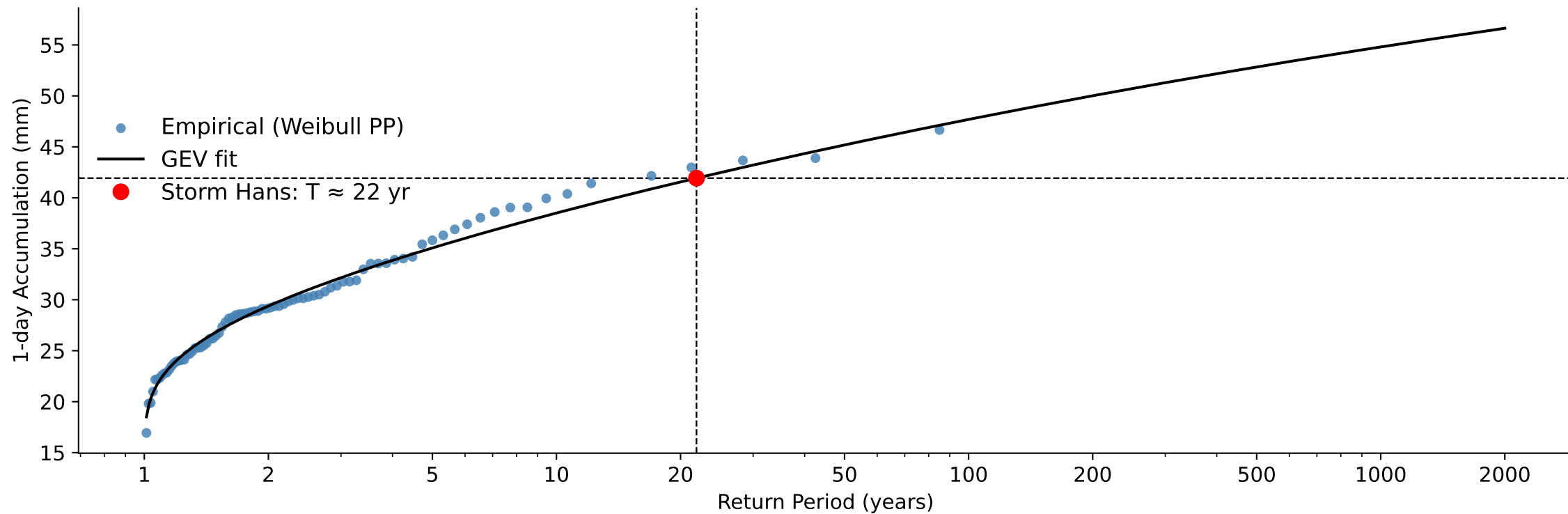
B) Weighted Catchment 1-day Accumulated Precipitation, Return Period Storm Hans: 22 year
