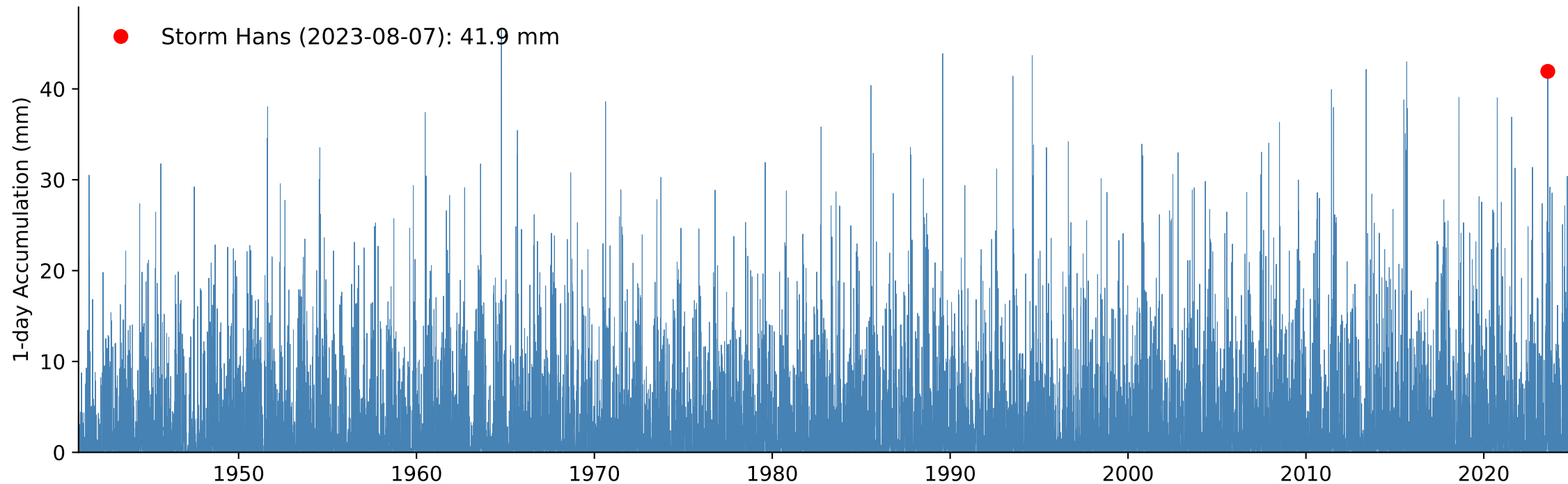
B) Weighted Catchment 1-day Accumulated Precipitation, Return Period Storm Hans: 22 year
