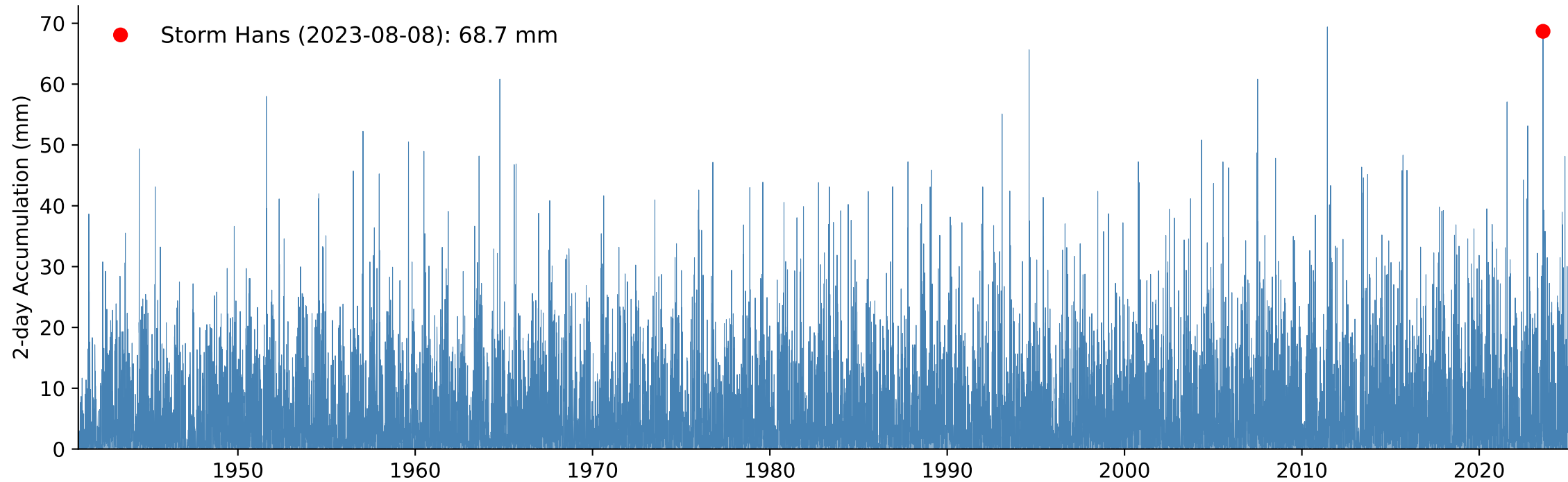
B) Weighted Catchment 2-day Accumulated Precipitation, Return Period Storm Hans: 105 year
