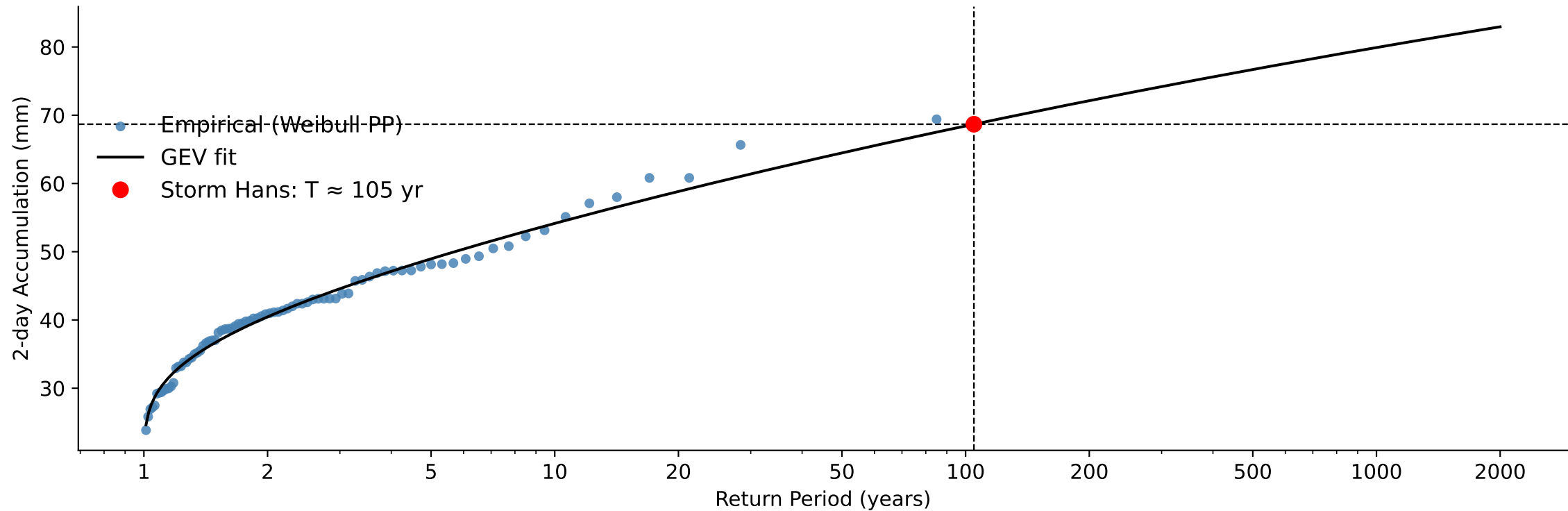
B) Weighted Catchment 2-day Accumulated Precipitation, Return Period Storm Hans: 105 year
