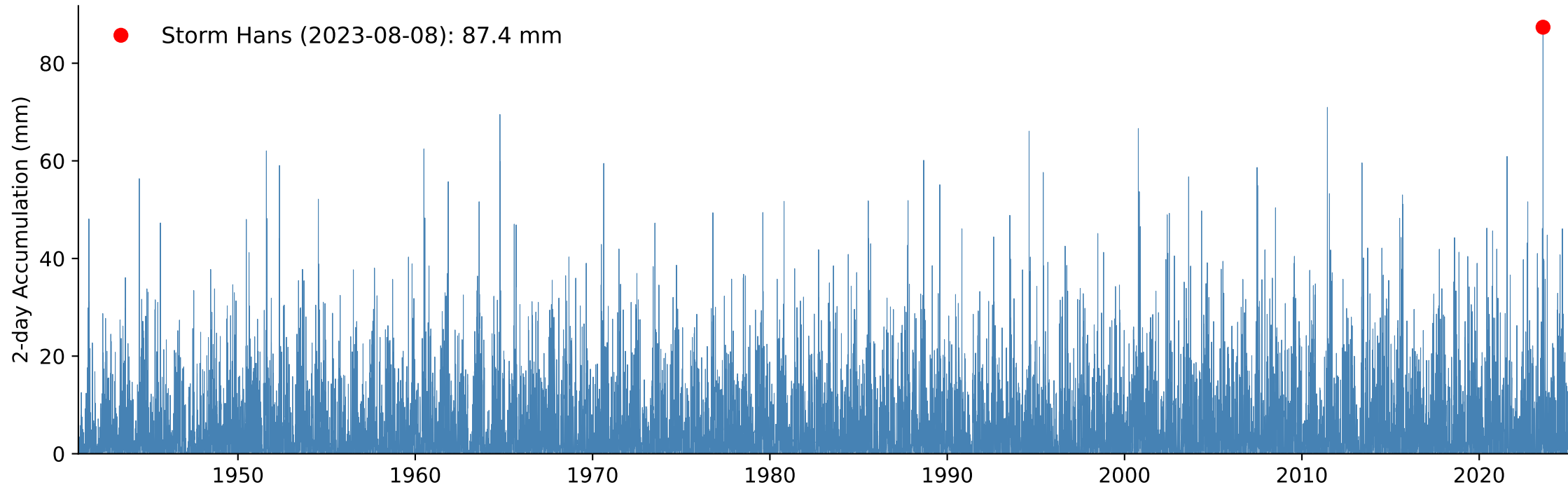
B) Weighted Catchment 2-day Accumulated Precipitation, Return Period Storm Hans: 172 year
