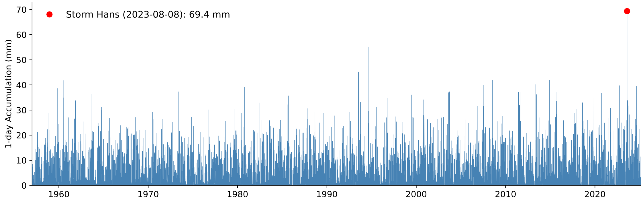
B) Weighted Catchment 1-day Accumulated Precipitation, Return Period Storm Hans: 196 year
