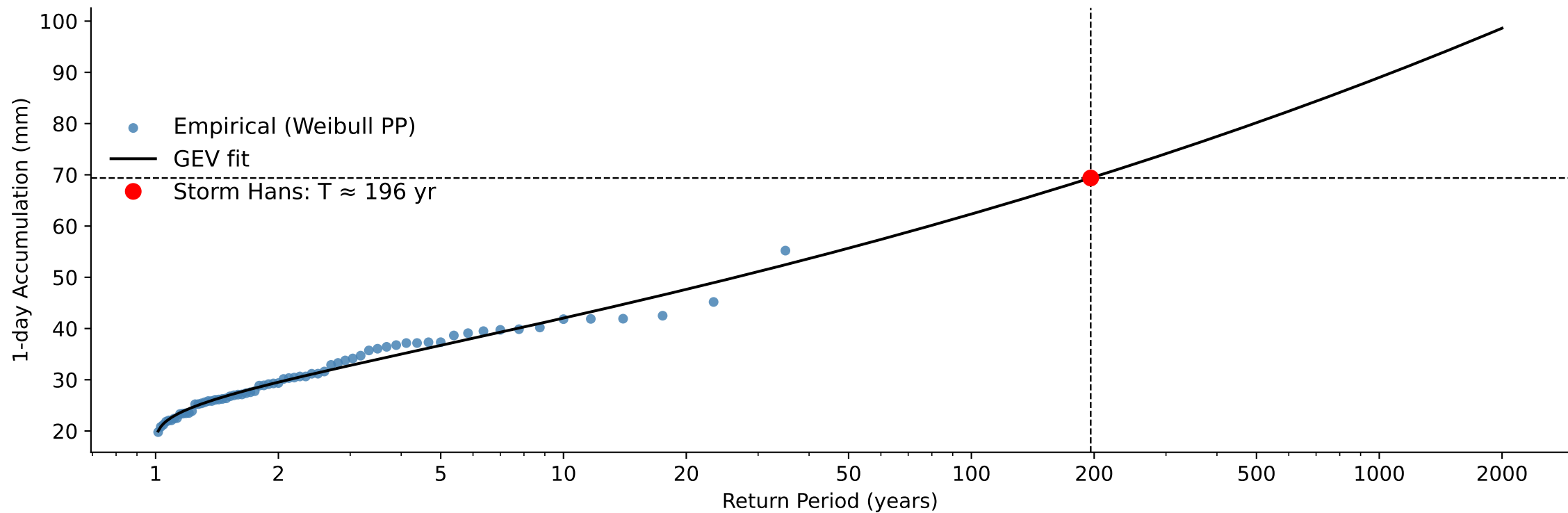
B) Weighted Catchment 1-day Accumulated Precipitation, Return Period Storm Hans: 196 year
