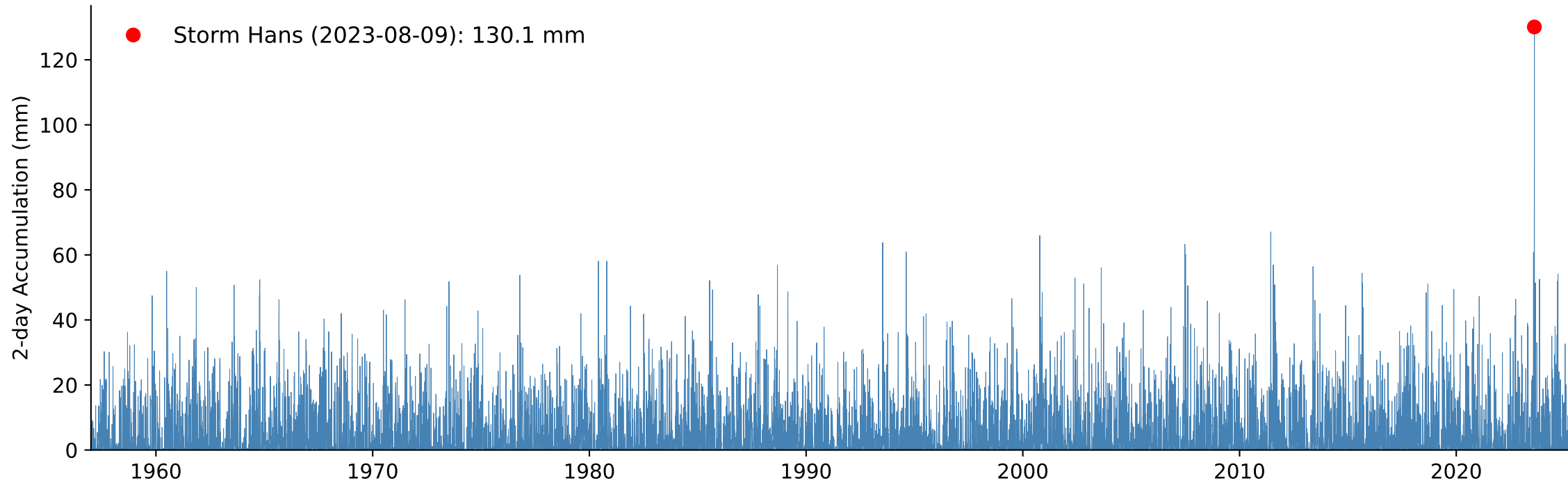
B) Weighted Catchment 2-day Accumulated Precipitation, Return Period Storm Hans: 1172 year
