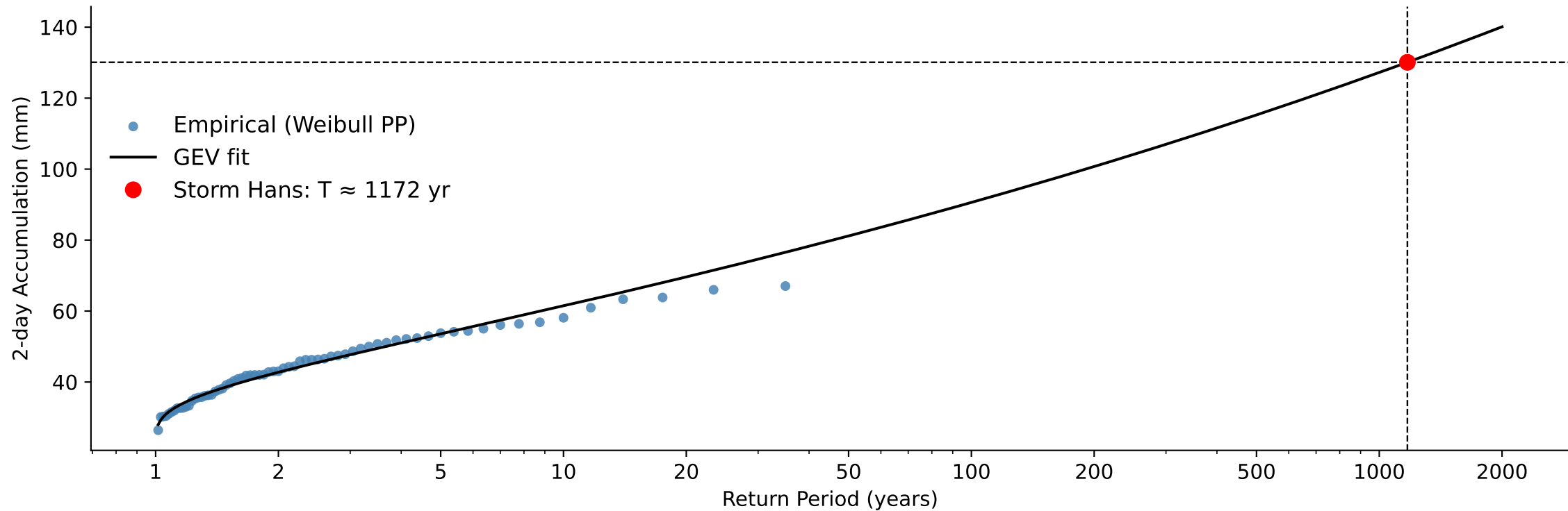
B) Weighted Catchment 2-day Accumulated Precipitation, Return Period Storm Hans: 1172 year
