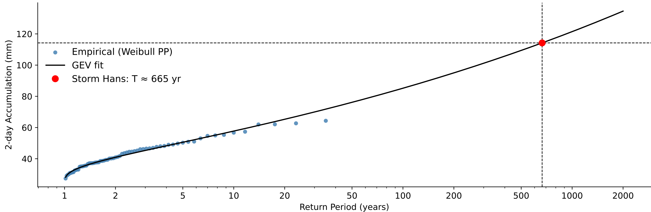
B) Weighted Catchment 2-day Accumulated Precipitation, Return Period Storm Hans: 665 year
