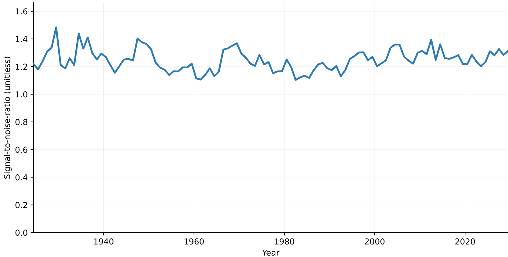
Signal-to-noise-ratio Compound (Precipitation and Soil Moisture) Hazard for Regine Drammen + Glomma from 1920-2034
