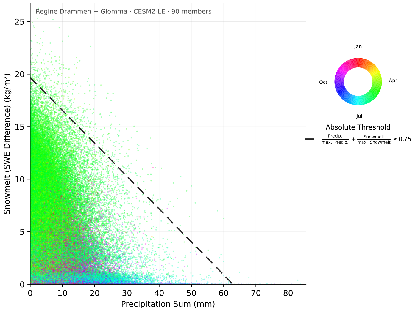
Joint Distribution of 2-Day Precipitation Sum and 2-Day Snowmelt (SWE Difference), 1995-2024
