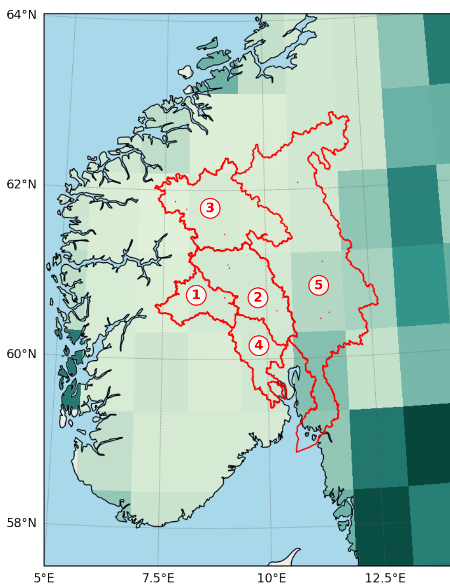
CESM2-LE / 0.942^\circ \times 1.25^\circ 100-Member Median
