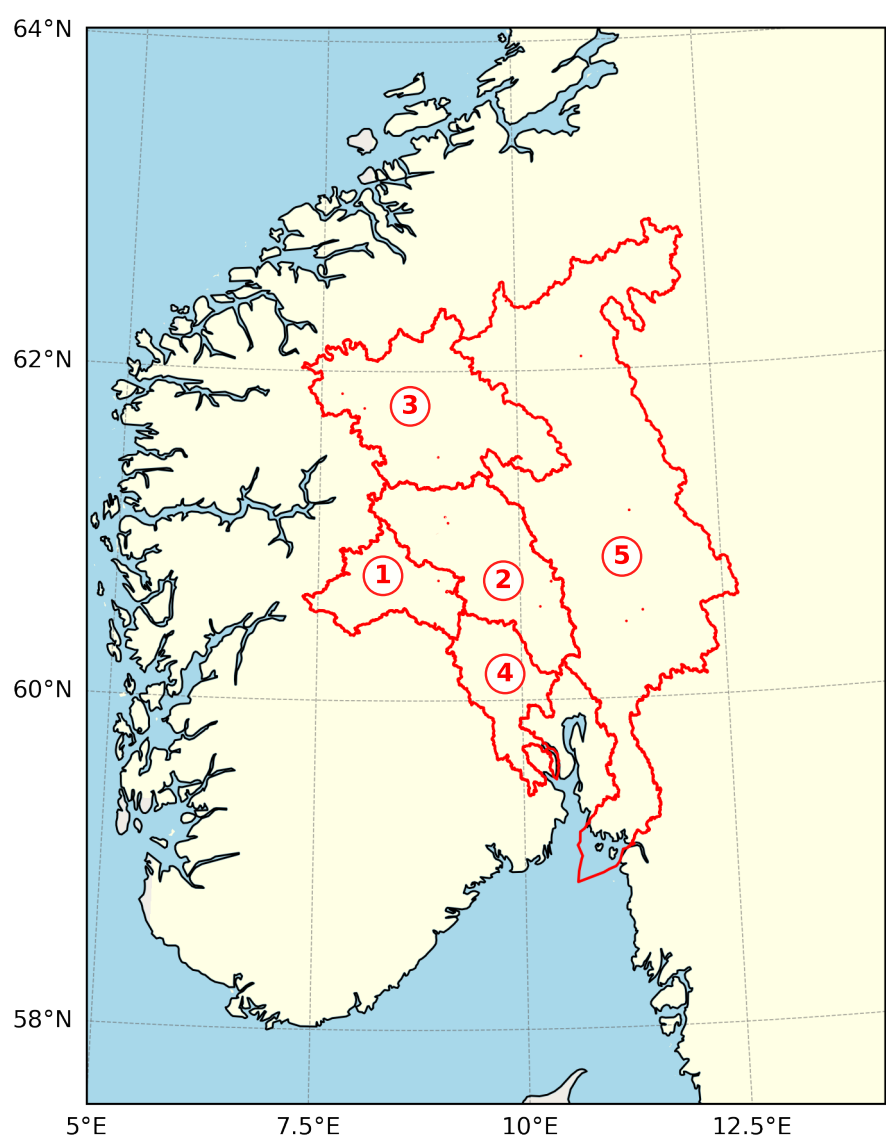
Autumn (SON)
