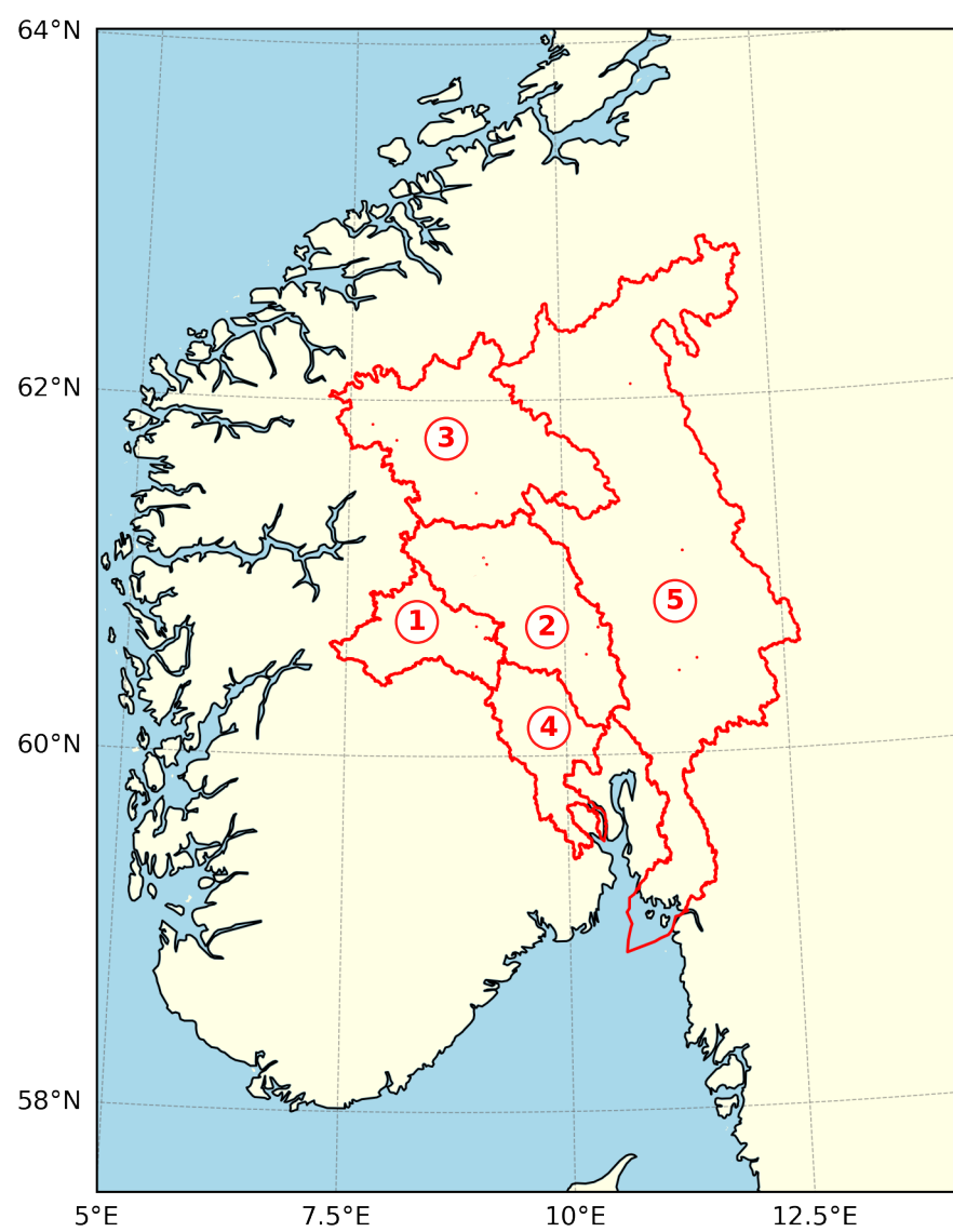
ERA5 Interpolated
