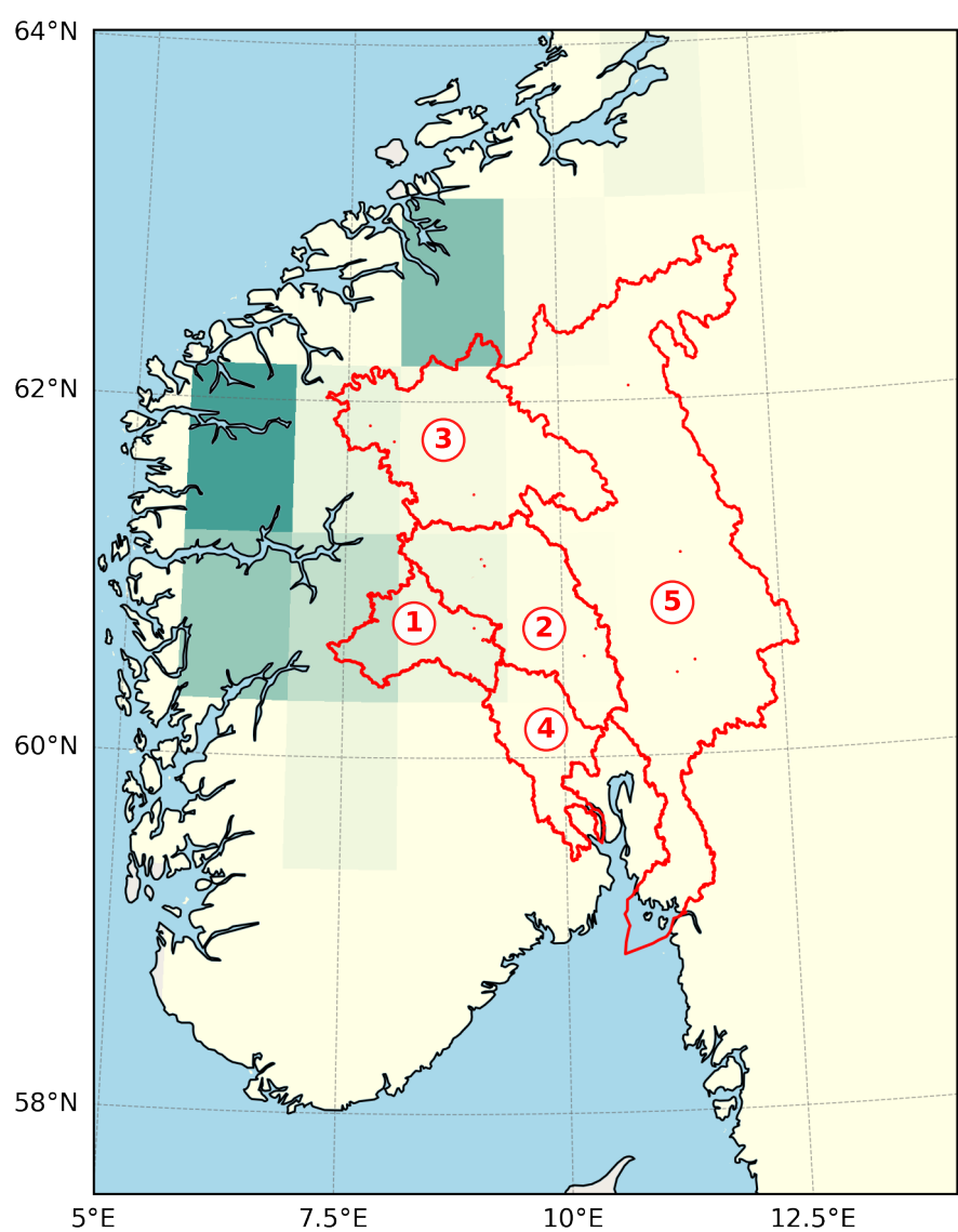
Spring (MAM)
