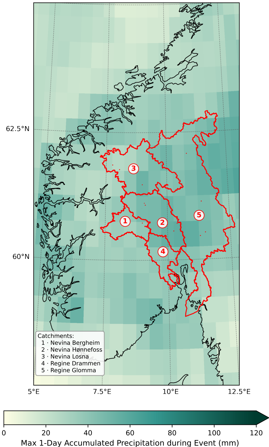
Storm Hans - Max 1-Day Precip. Envelope (7-9 Aug 2023): ERA5/0.5°x0.5°
