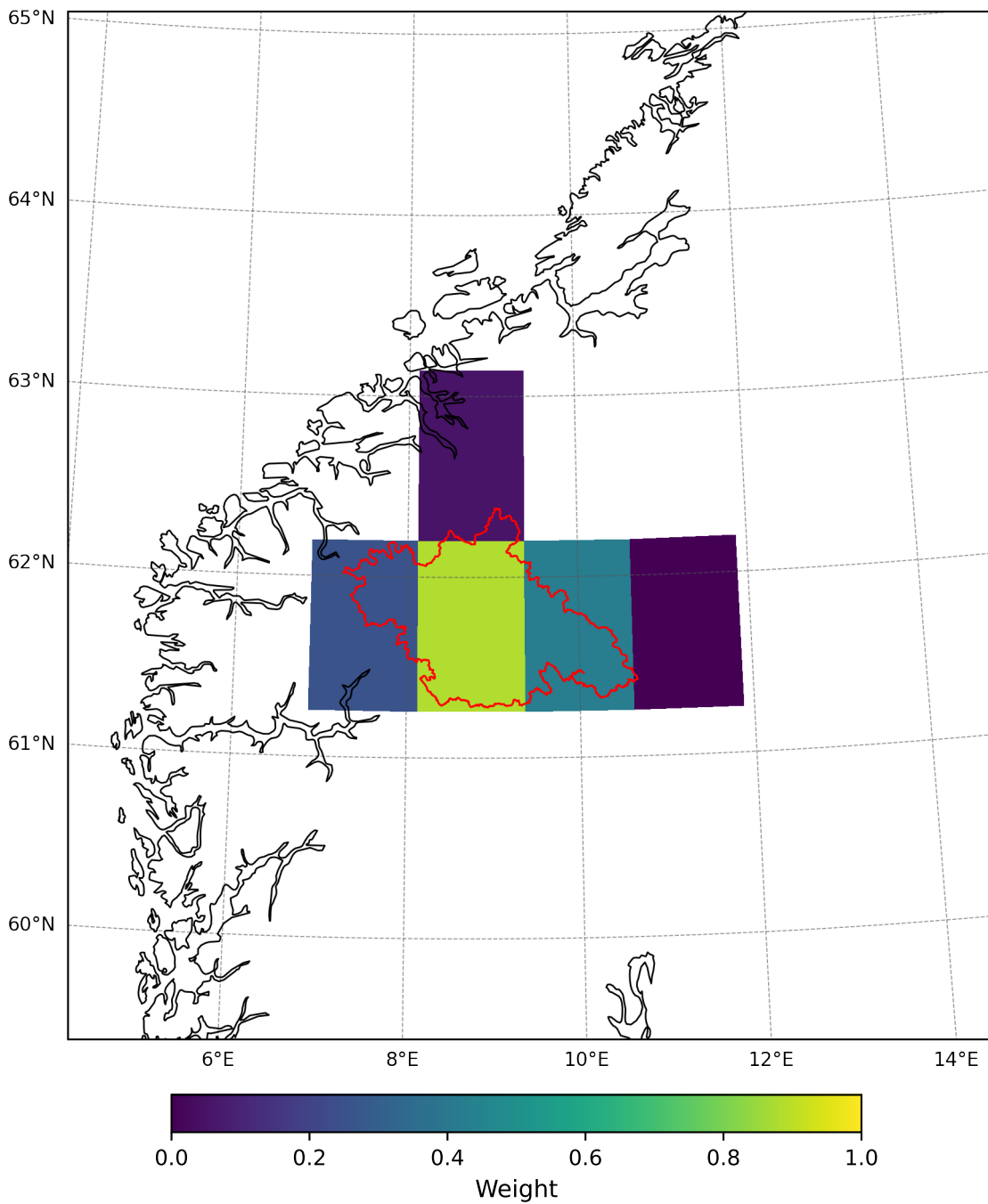
Catchment Weights: CESM2-LE/0.94x1.25 — Nevina Losna
