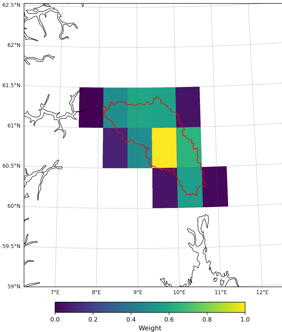
Catchment Weights: GFDL-SPEAR/0.5x0.625 — Nevina Hønnefoss
