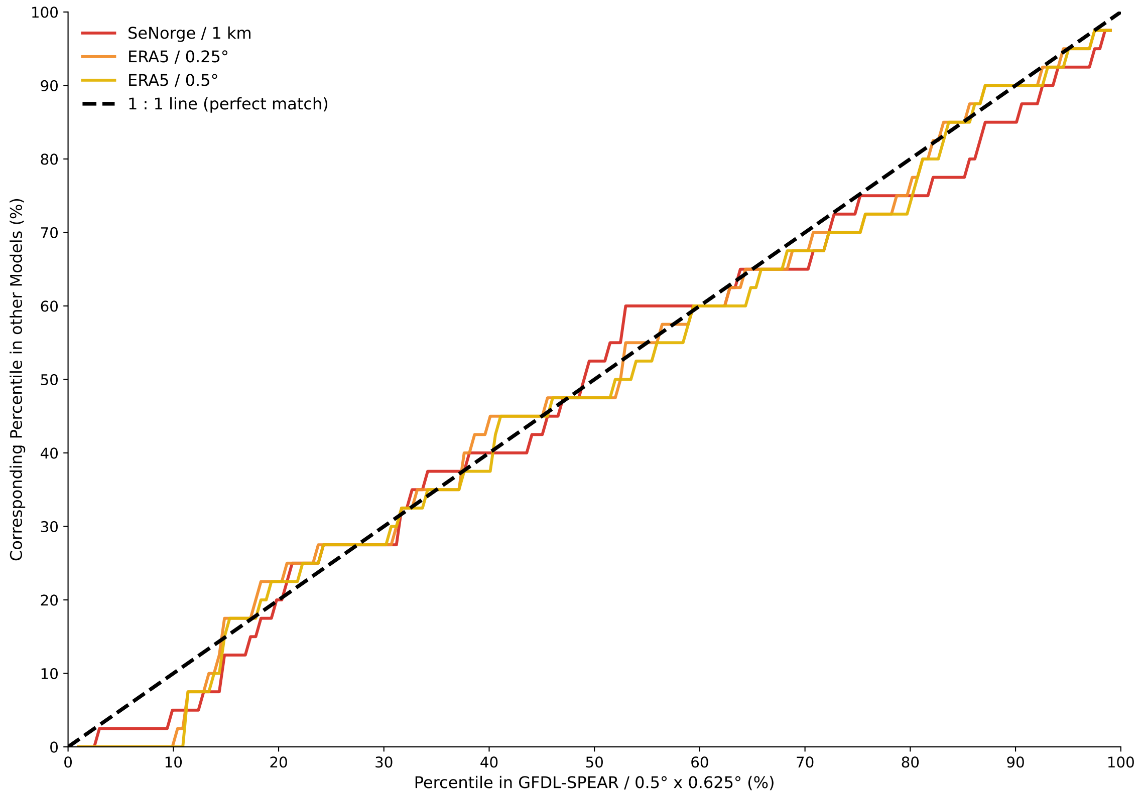
Percentile Mapping of Annual Maximal 2-day Accumulated Precipitation — Regime Glomma
