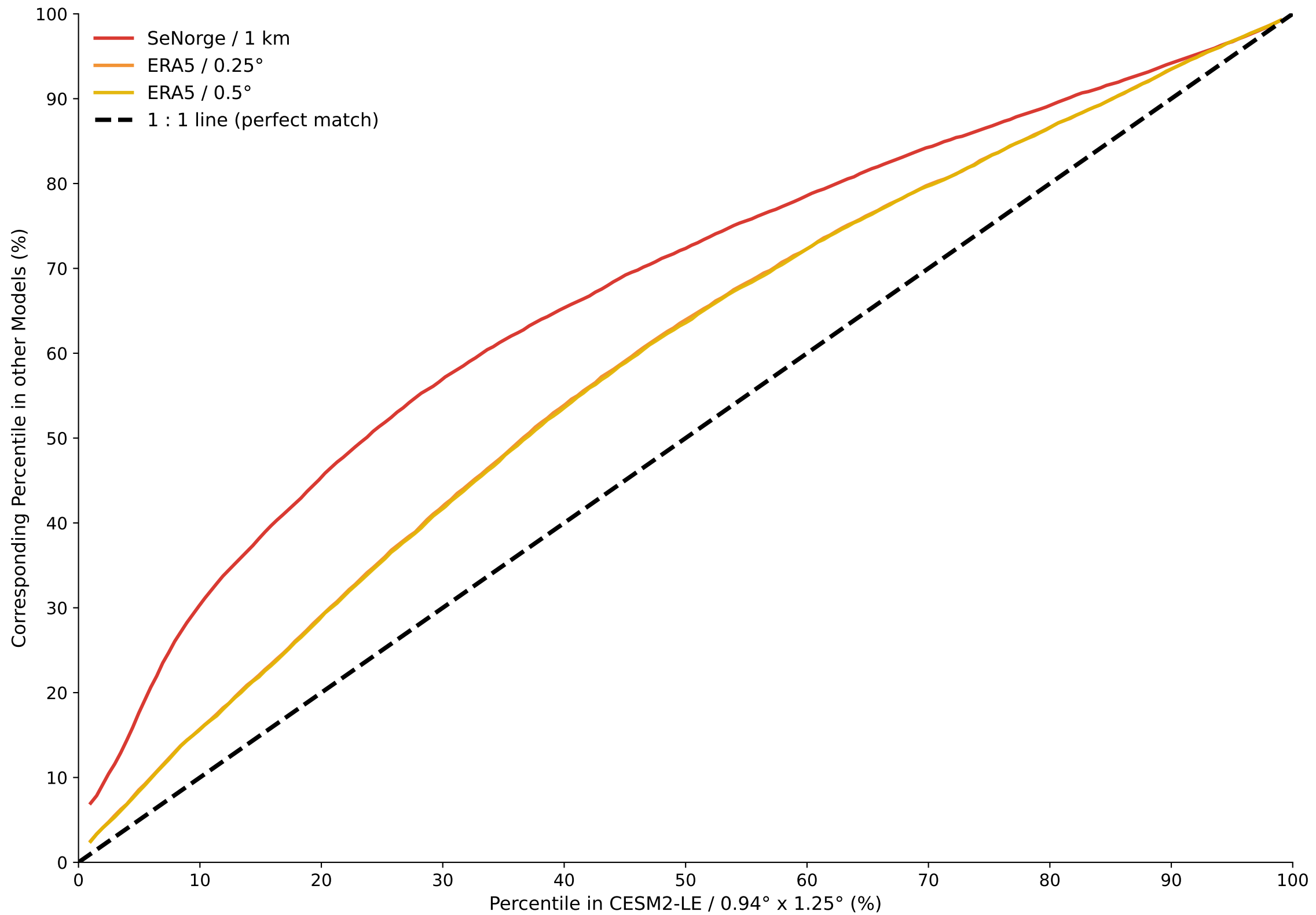
Percentile Mapping of Daily 1-day Accumulated Precipitation — Nevina Losna
