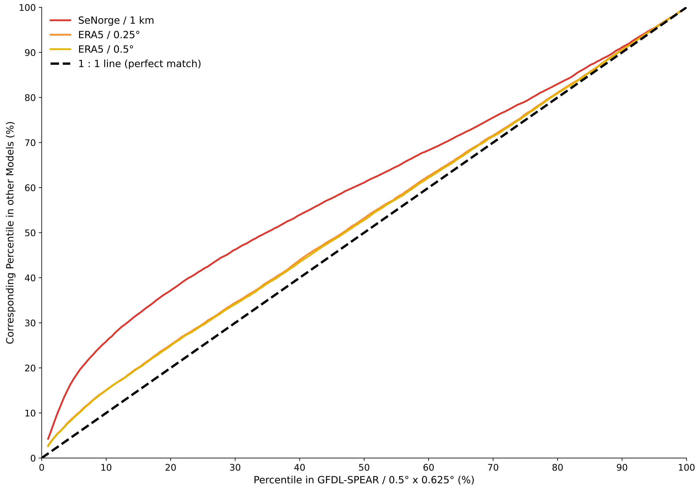
Percentile Mapping of Daily 1-day Accumulated Precipitation — Regime Glomma
