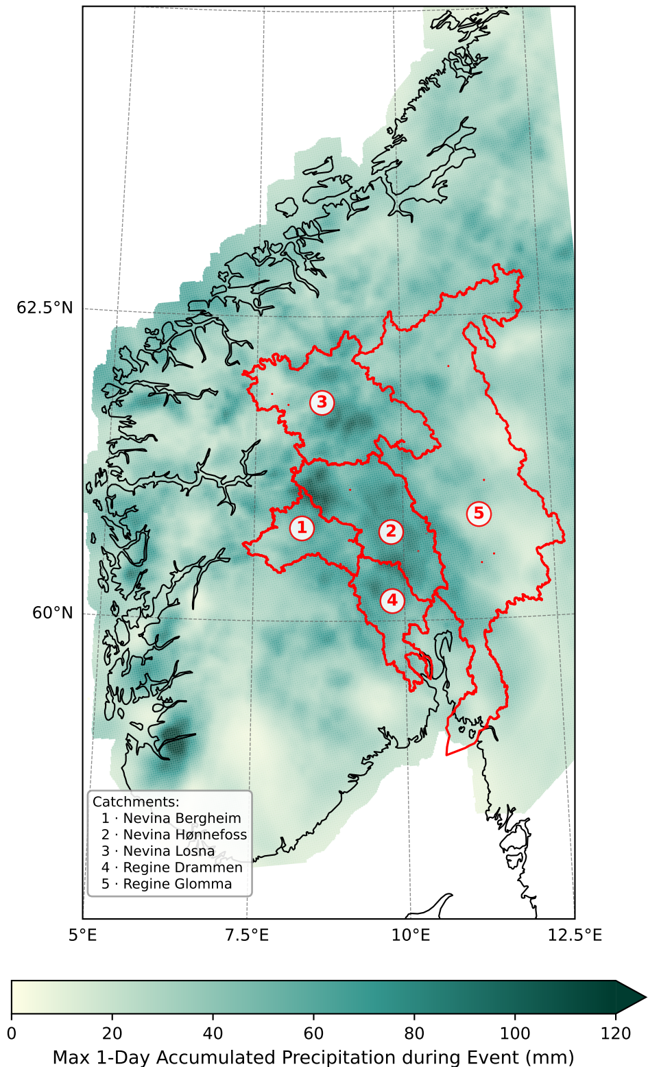
Storm Hans - Max 1-Day Precip. Envelope (7-9 Aug 2023): SeNorge/1kmx1km
